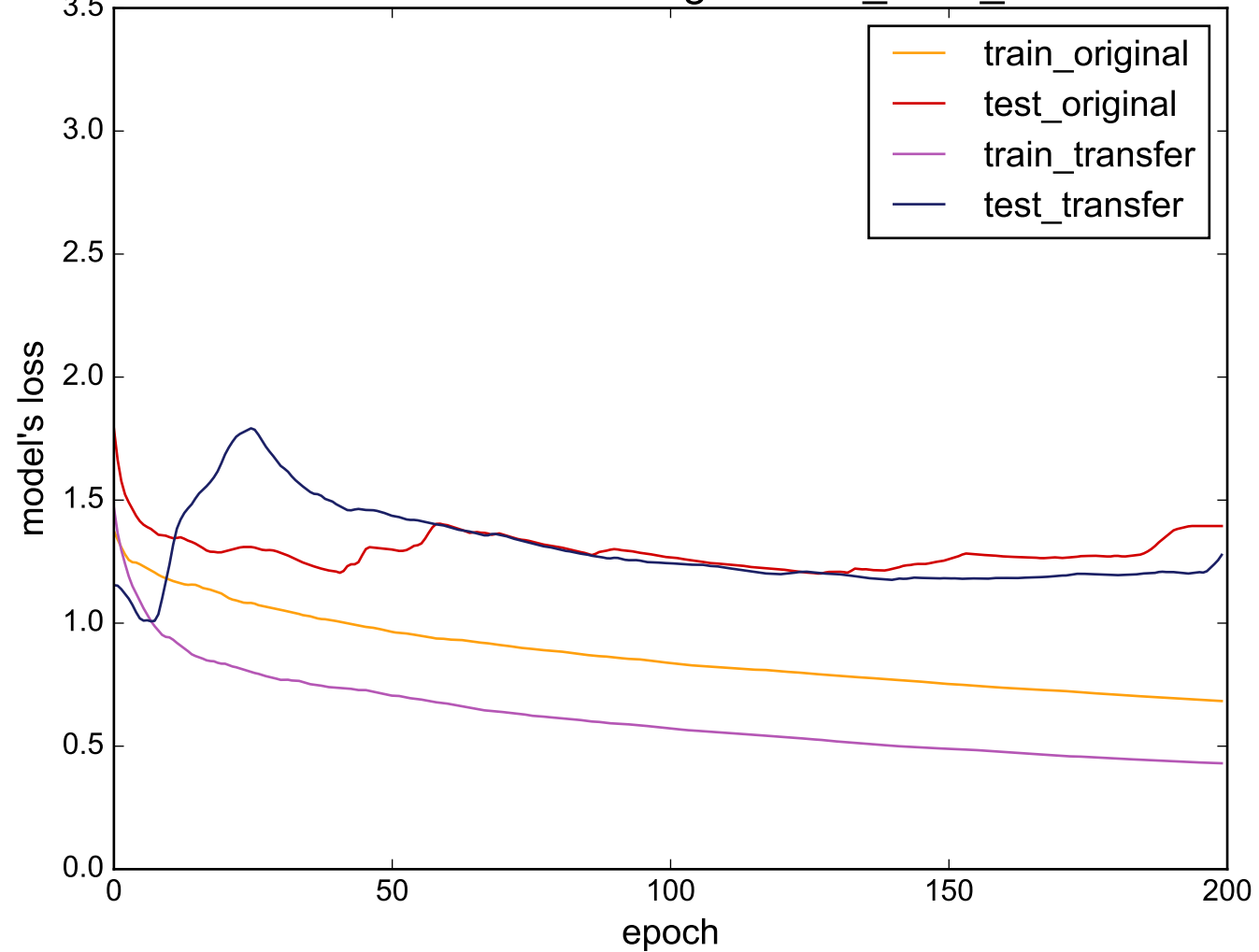
Source: OSULeaf - Target: CinC_ECG_torso
