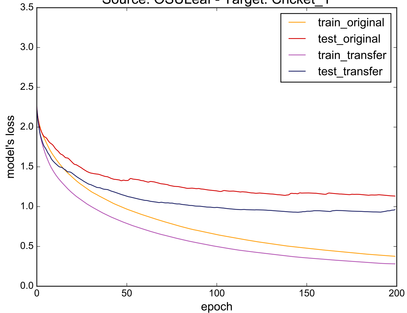
Source: OSULeaf - Target: Cricket_Y
