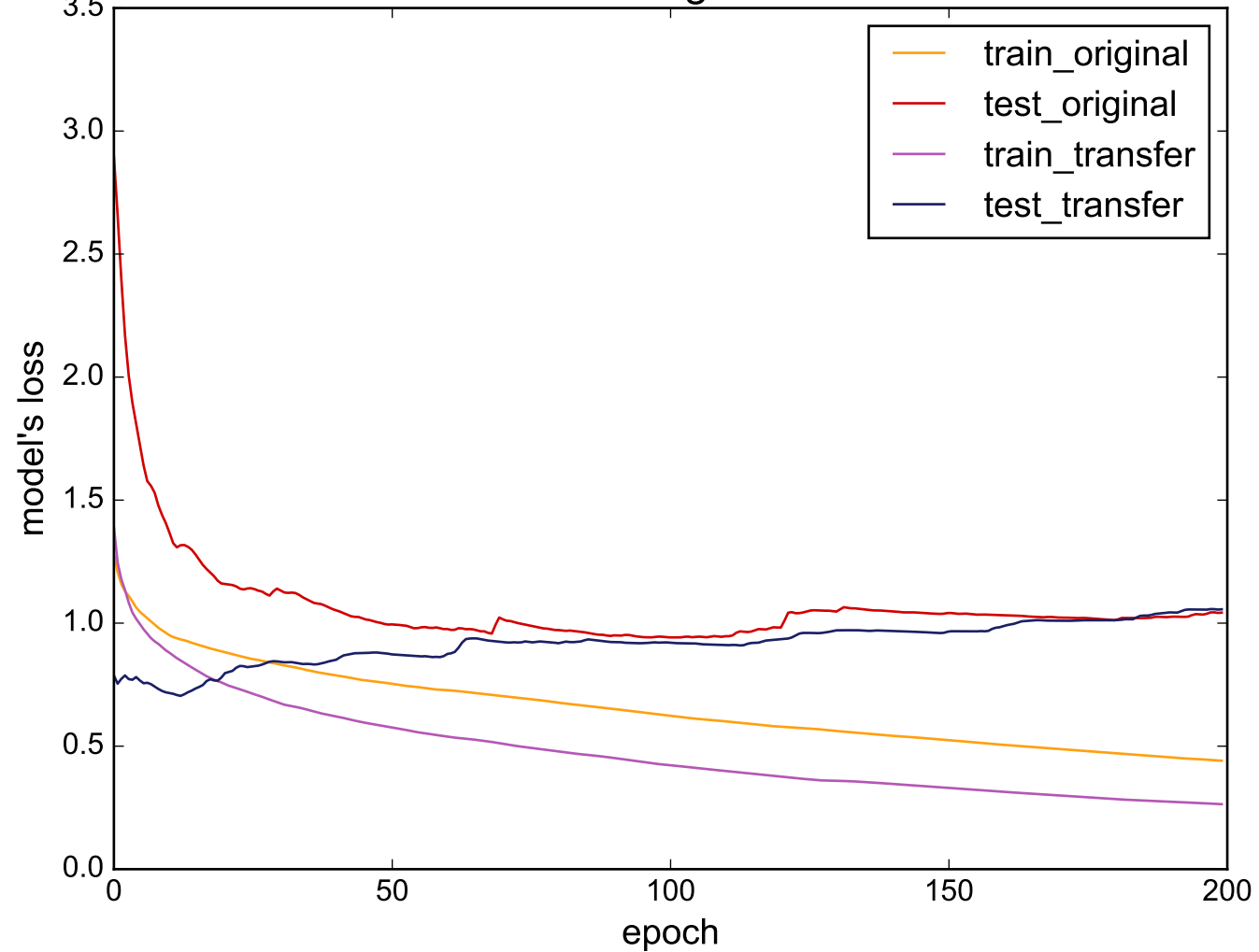
Source: OSULeaf - Target: DistalPhalanxTW
