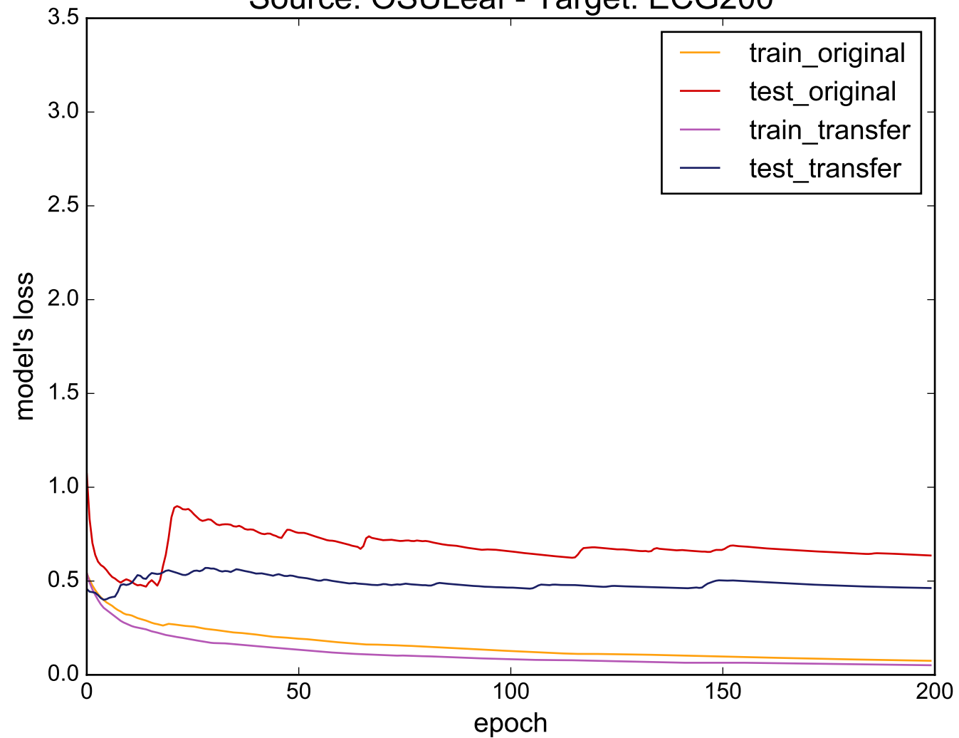
Source: OSULeaf - Target: ECG200
