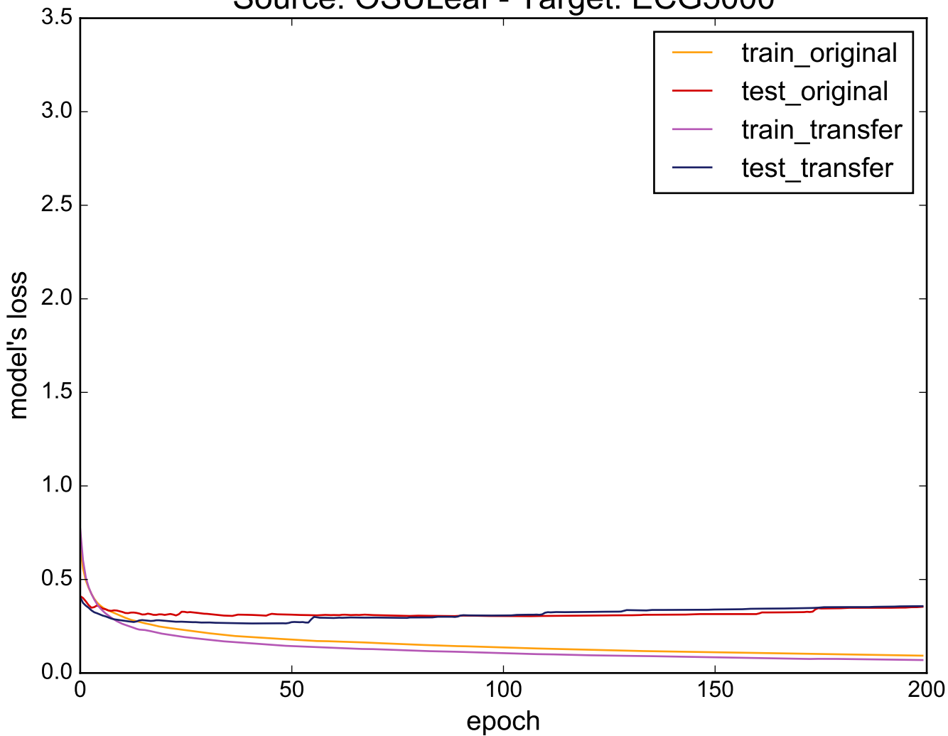
Source: OSULeaf - Target: ECG5000
