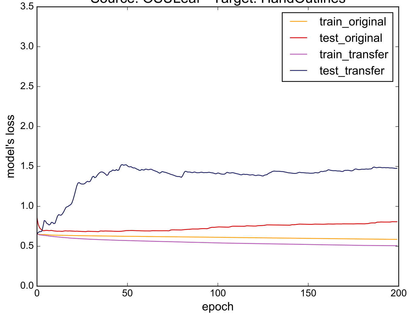
Source: OSULeaf - Target: HandOutlines
