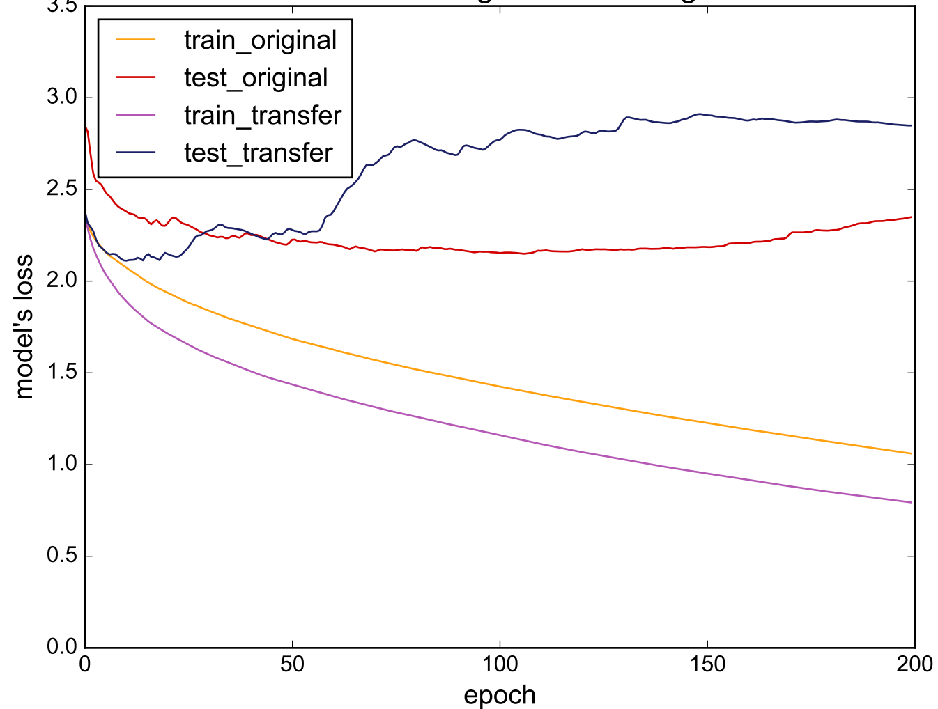
Source: OSULeaf - Target: InsectWingbeatSound
