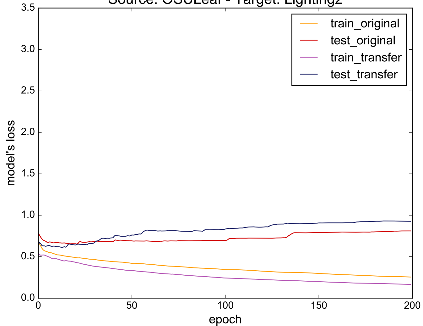
Source: OSULeaf - Target: Lighting2
