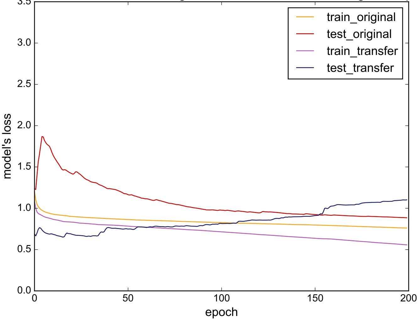
Source: OSULeaf - Target: MiddlePhalanxOutlineAgeGroup
