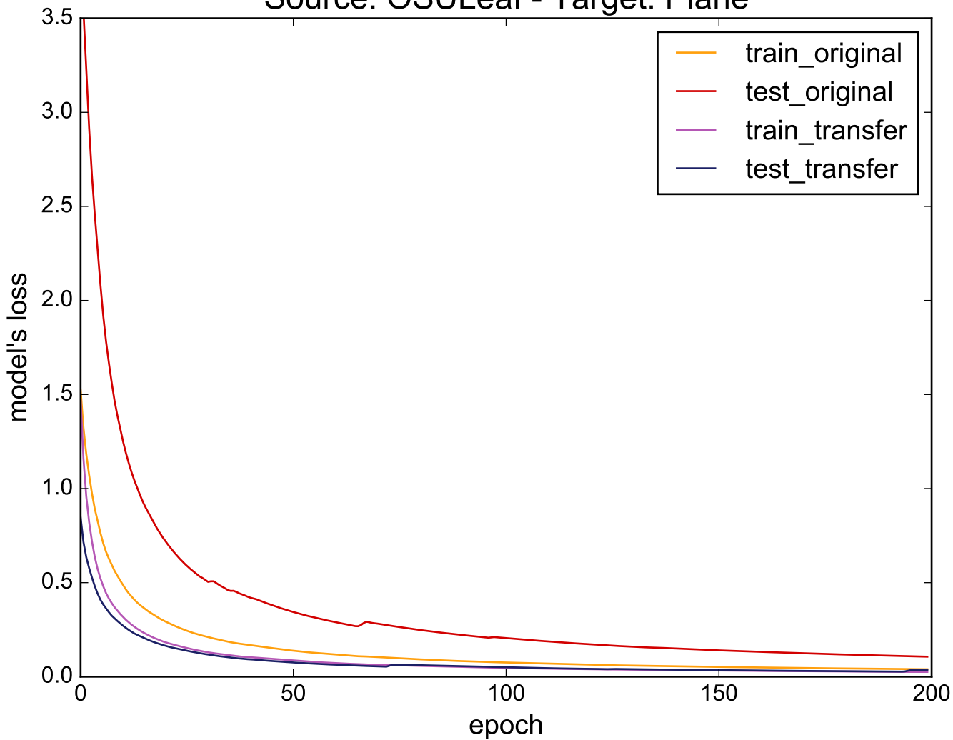
Source: OSULeaf - Target: Plane
