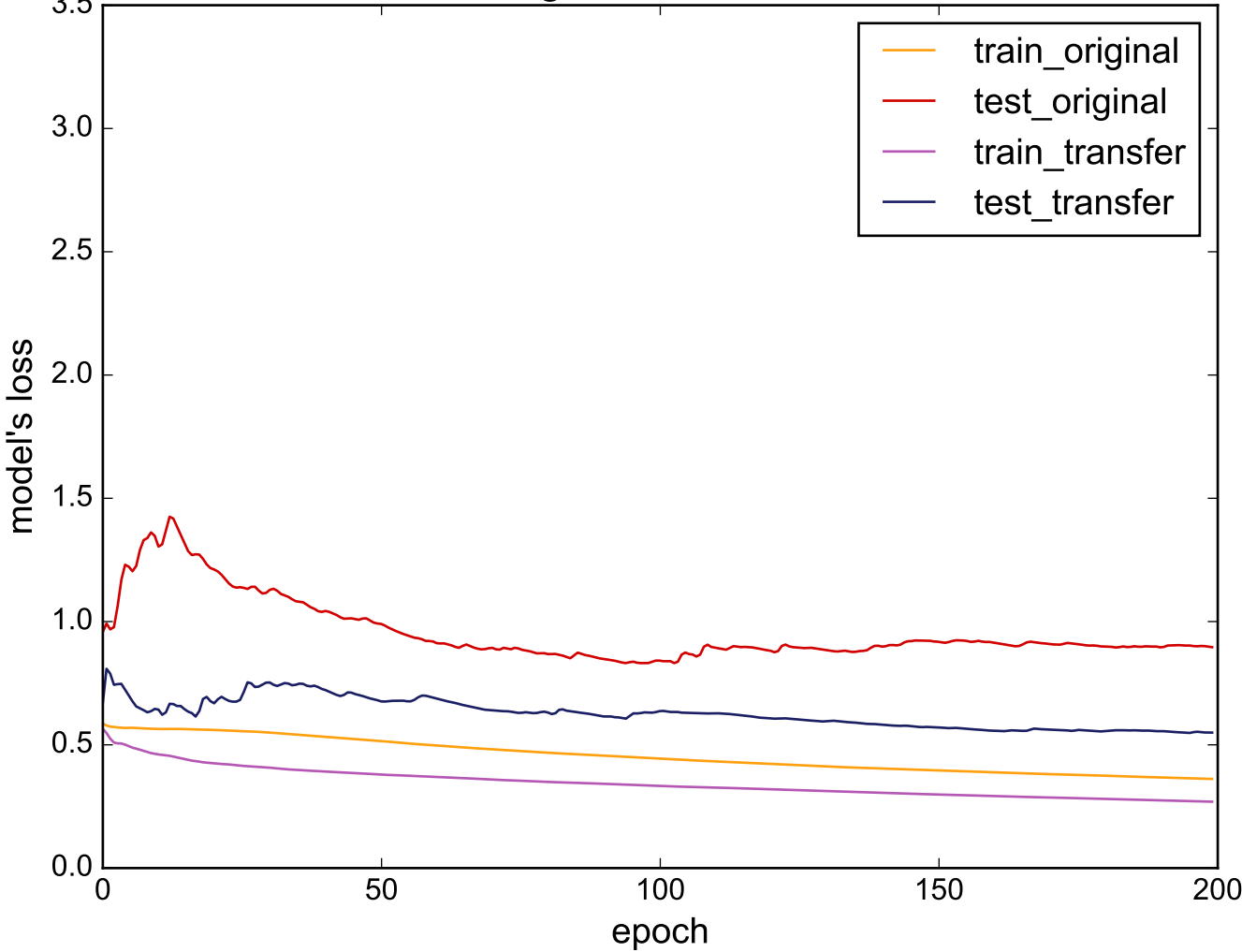
Source: OSULeaf - Target: ProximalPhalanxOutlineCorrect
