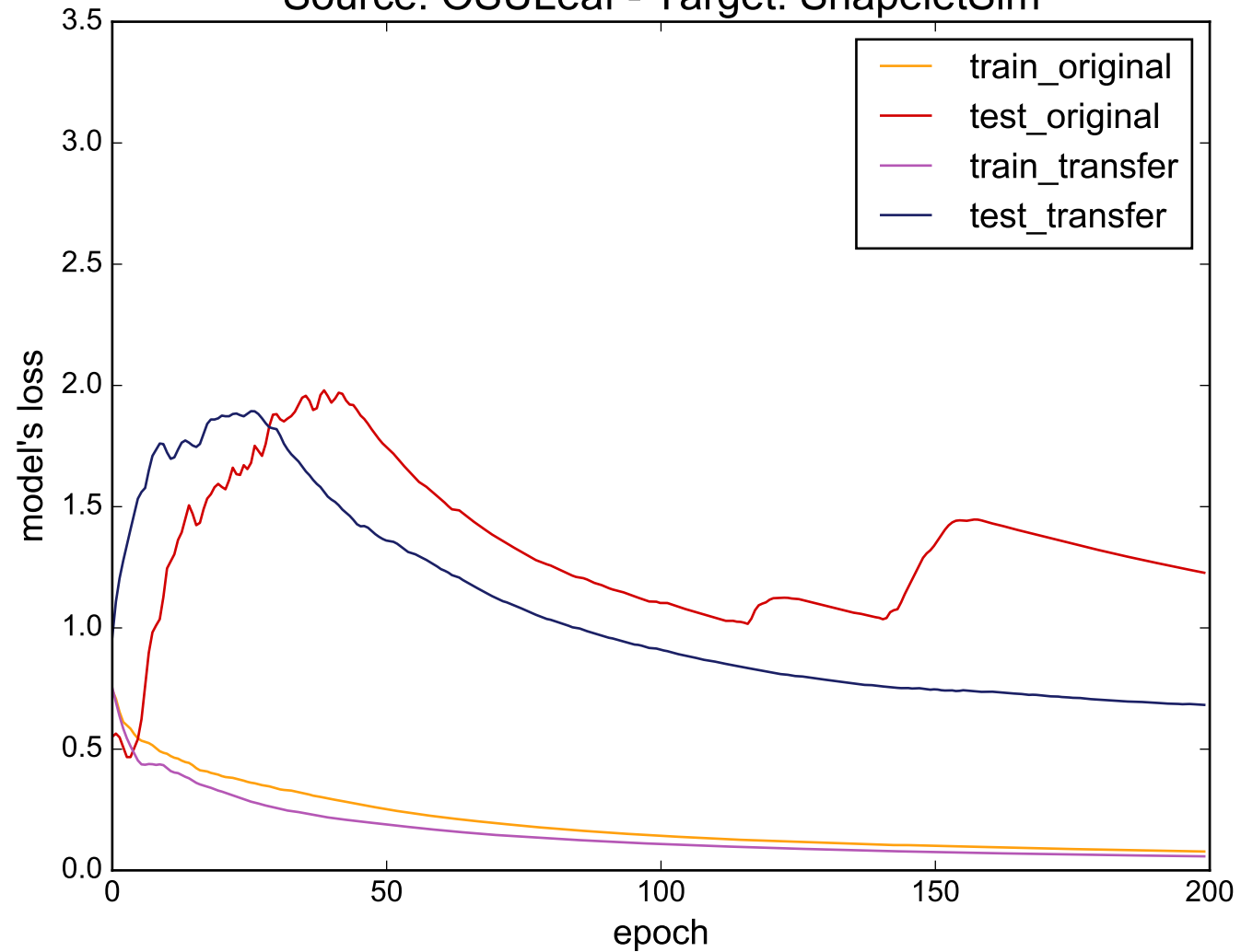
Source: OSULeaf - Target: ShapeletSim
