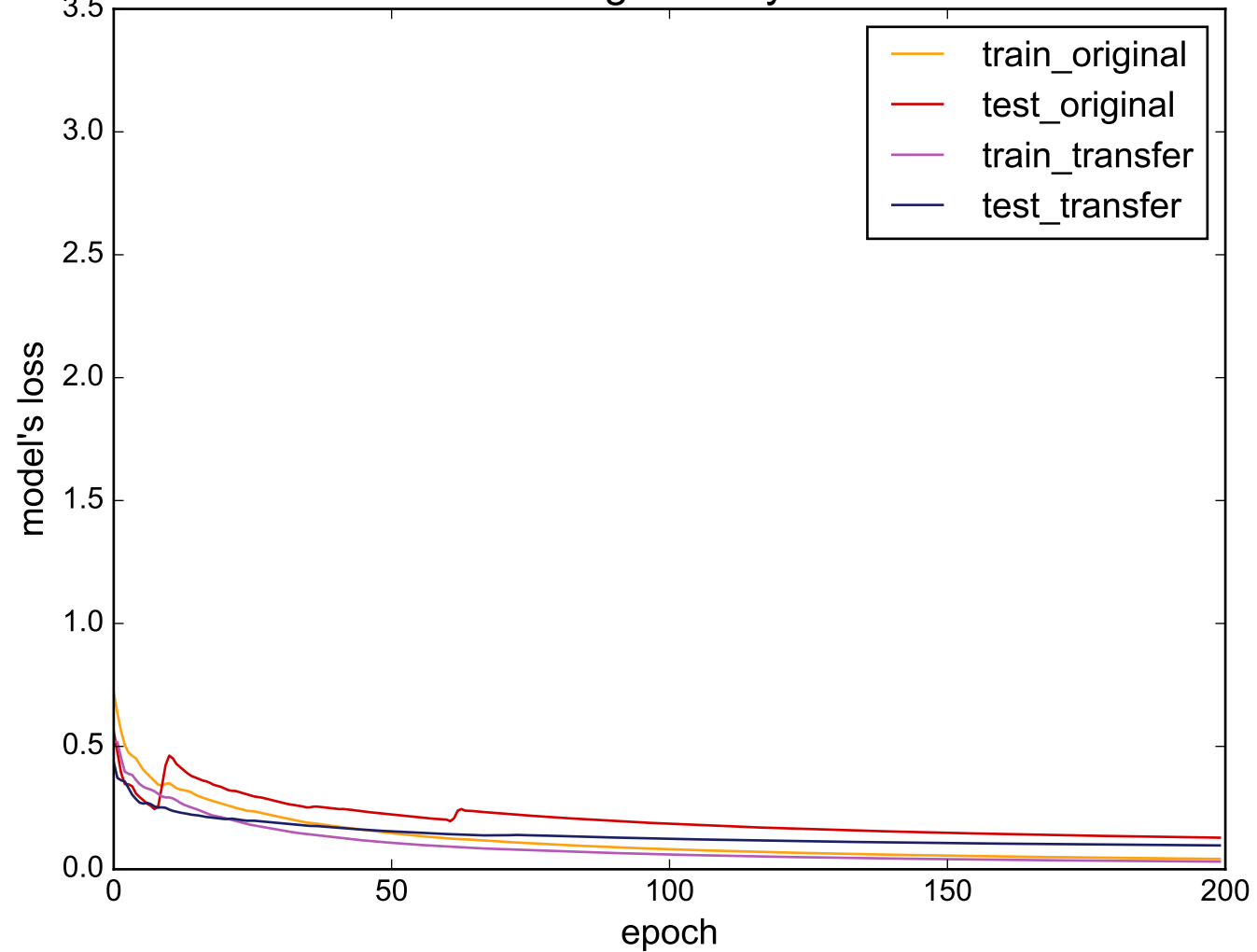
Source: OSULeaf - Target: SonyAIBORobotSurfaceII
