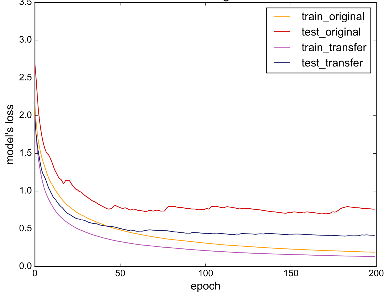
Source: OSULeaf - Target: SwedishLeaf
