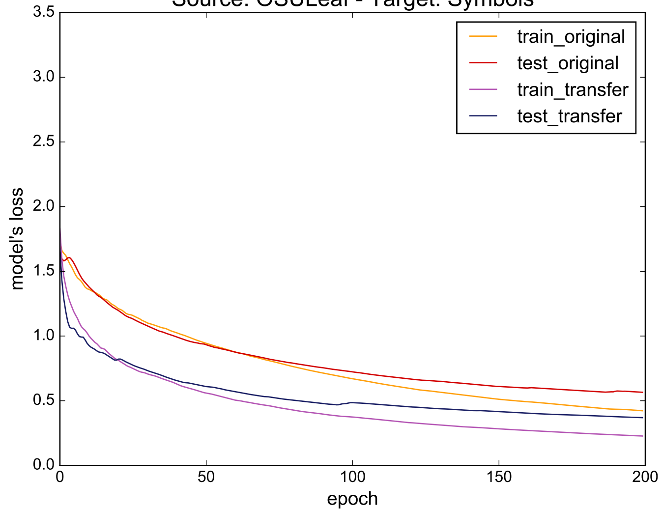
Source: OSULeaf - Target: Symbols
