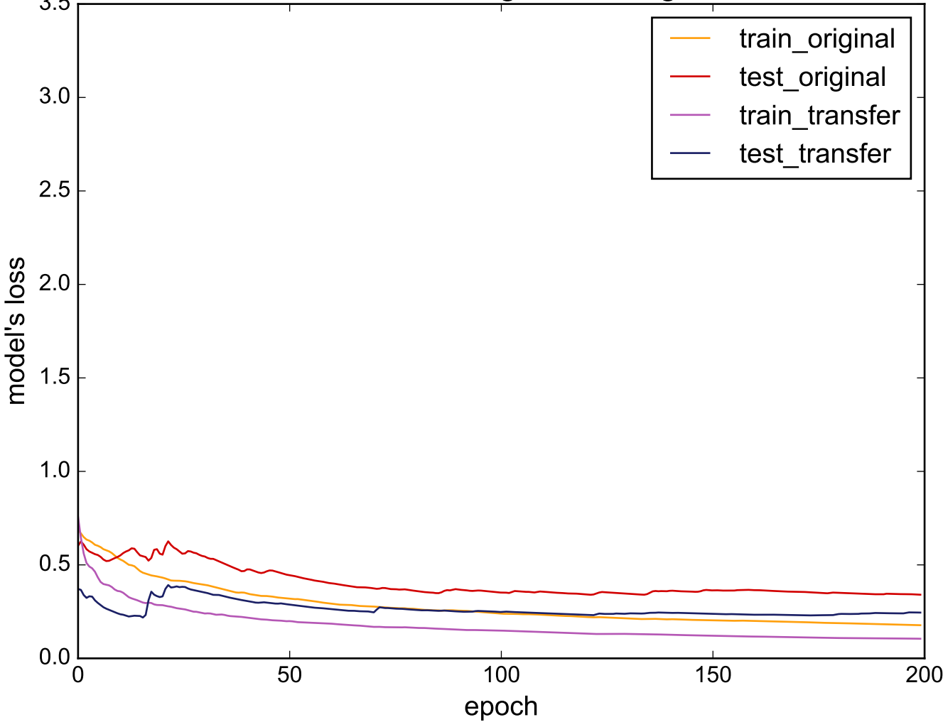
Source: OSULeaf - Target: ToeSegmentation1
