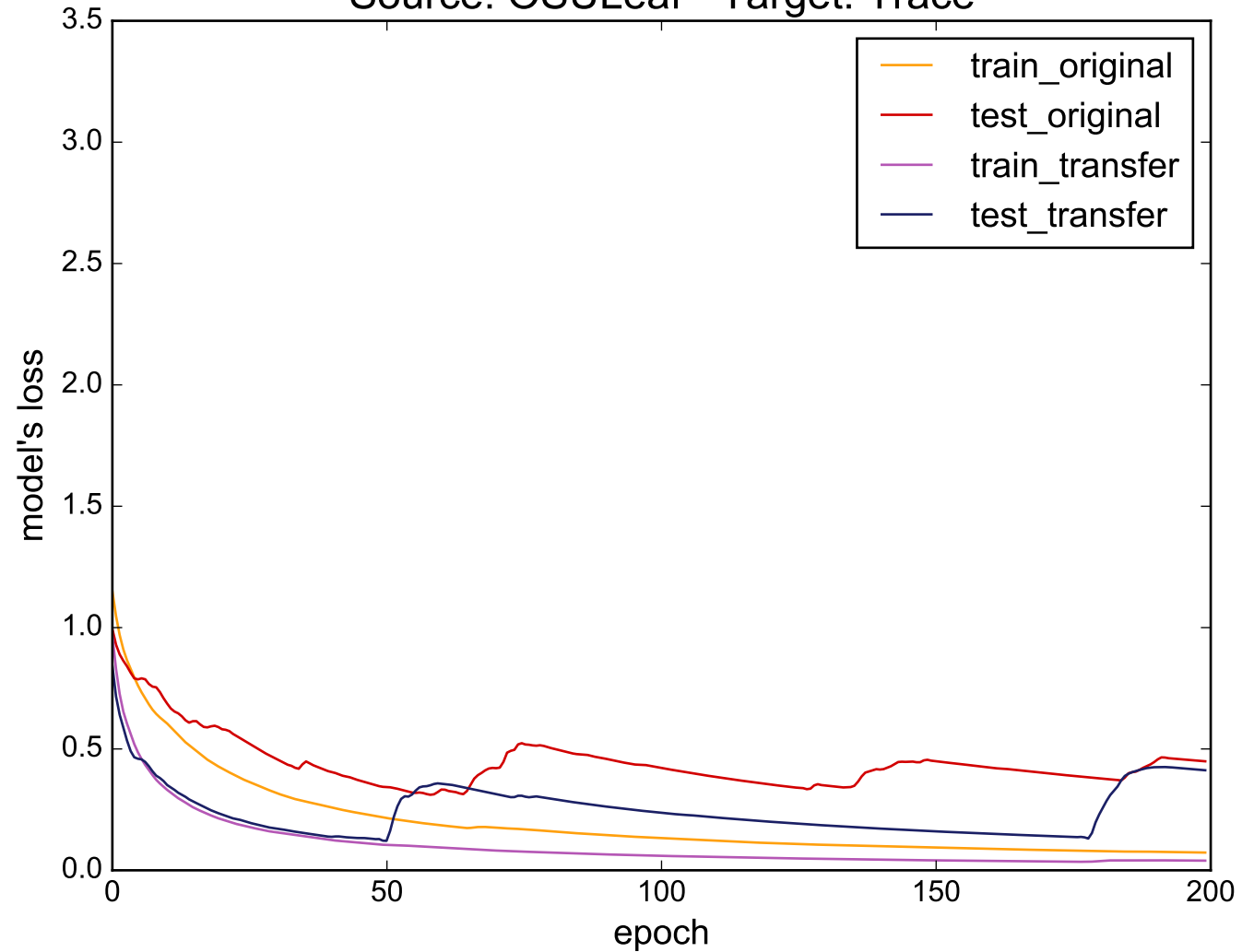
Source: OSULeaf - Target: Trace
