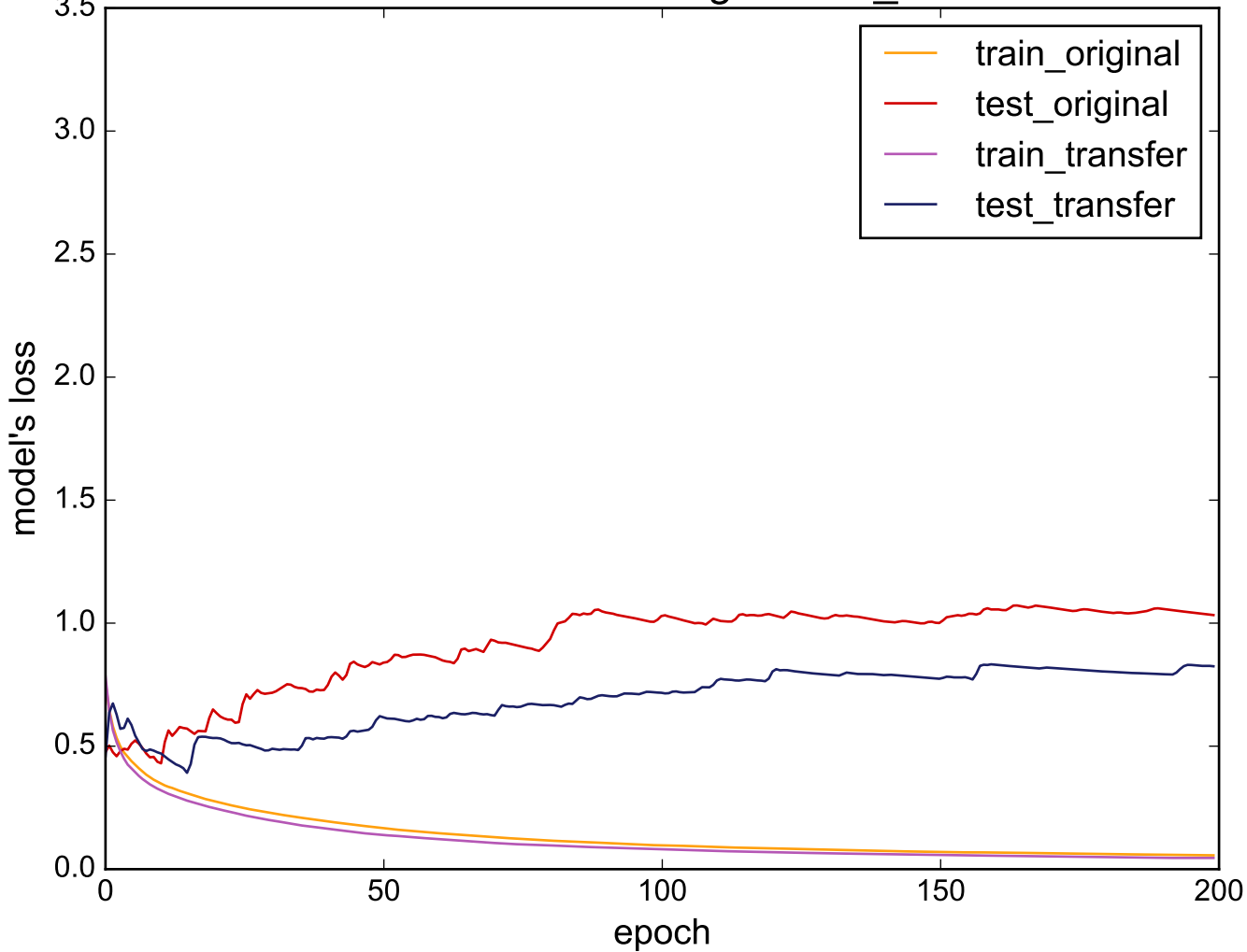
Source: OSULeaf - Target: Two_Patterns
