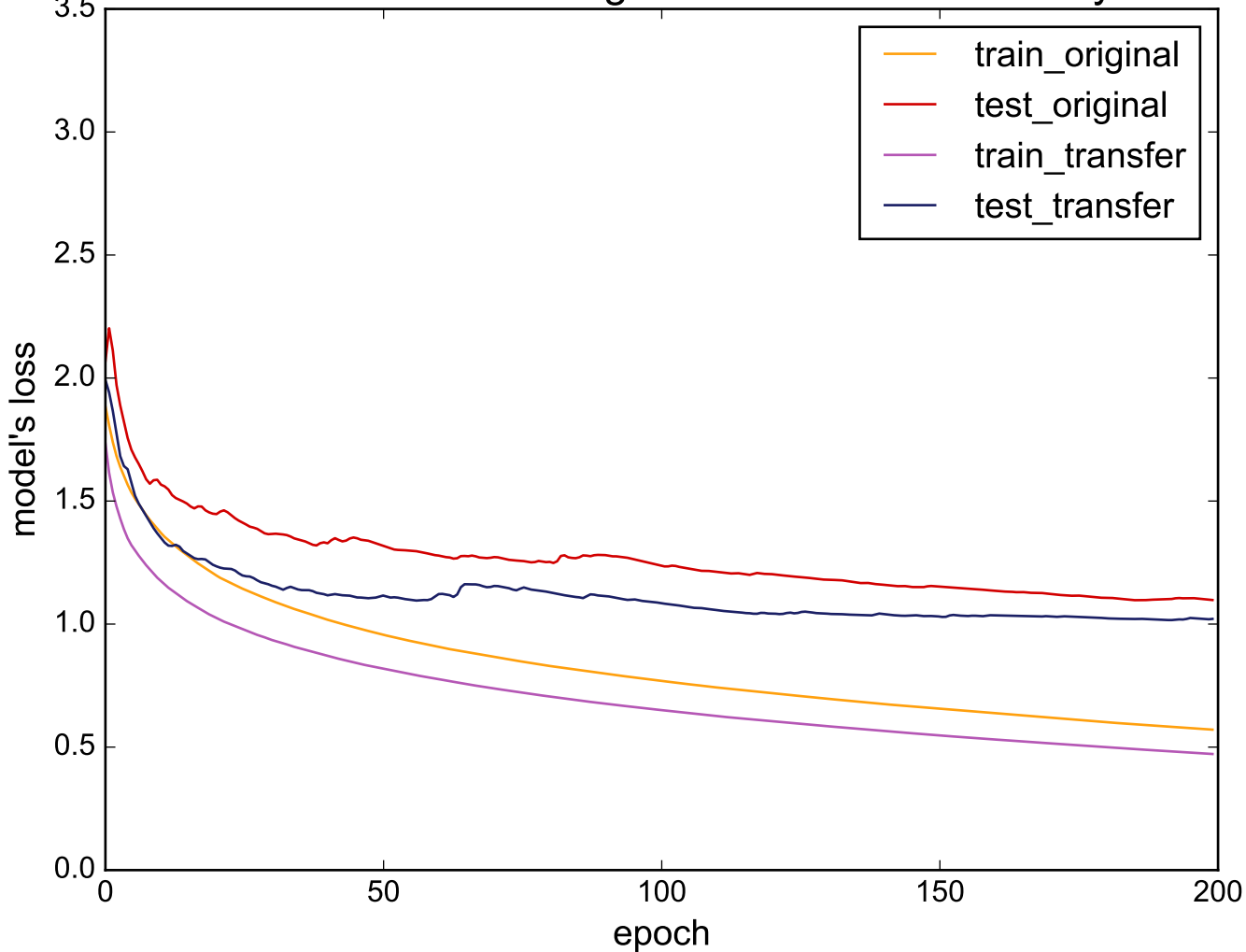
Source: OSULeaf - Target: UWaveGestureLibraryAll
