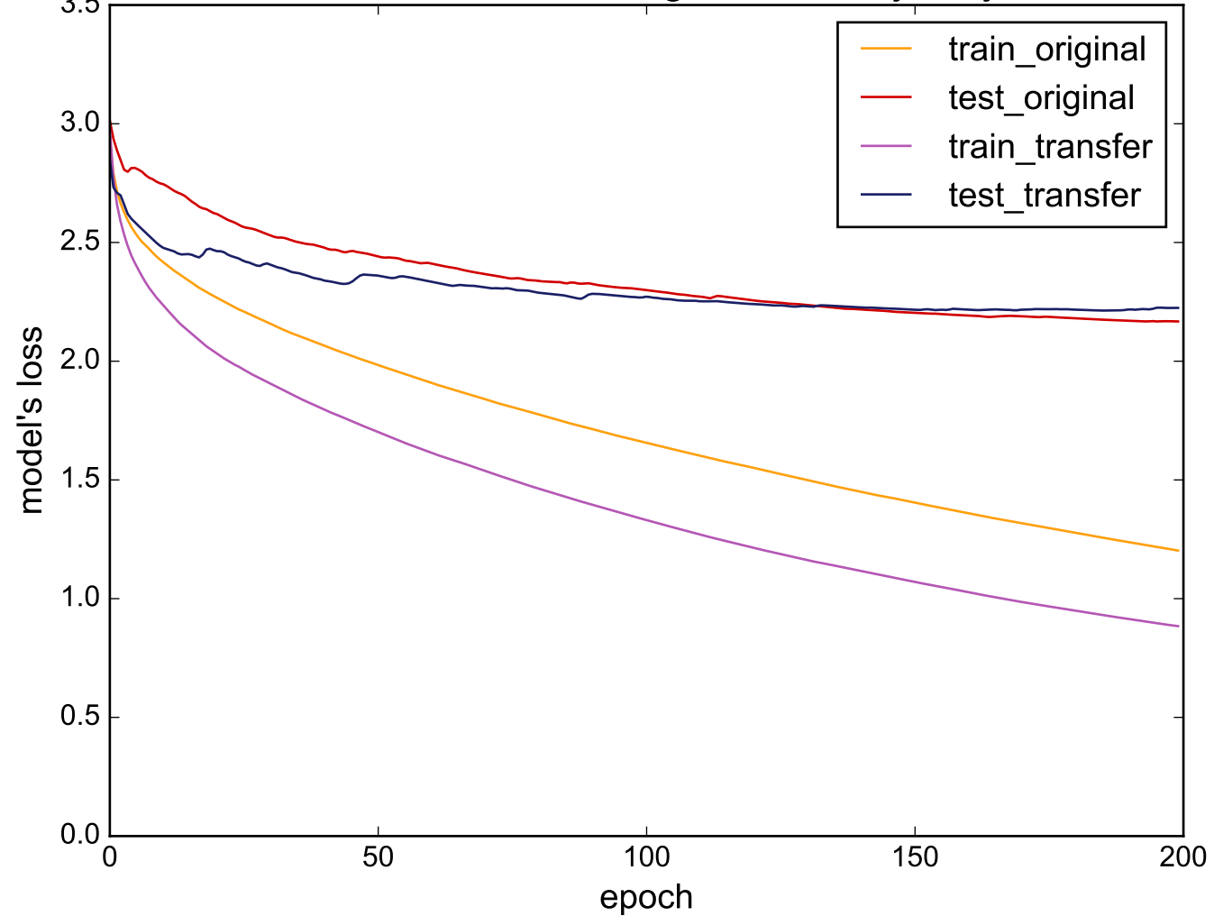
Source: OSULeaf - Target: WordsSynonyms
