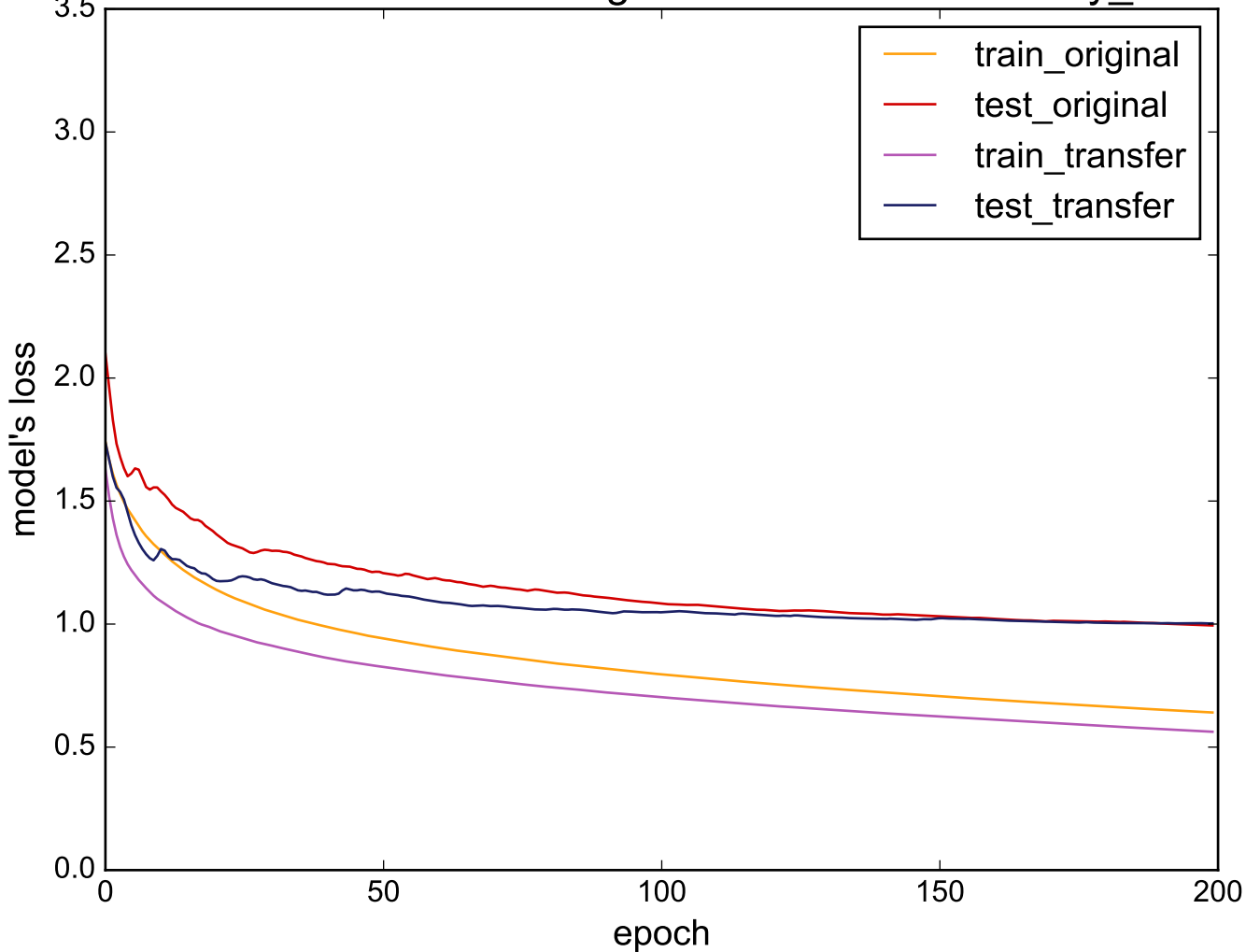
Source: OSULeaf - Target: uWaveGestureLibrary_Z
