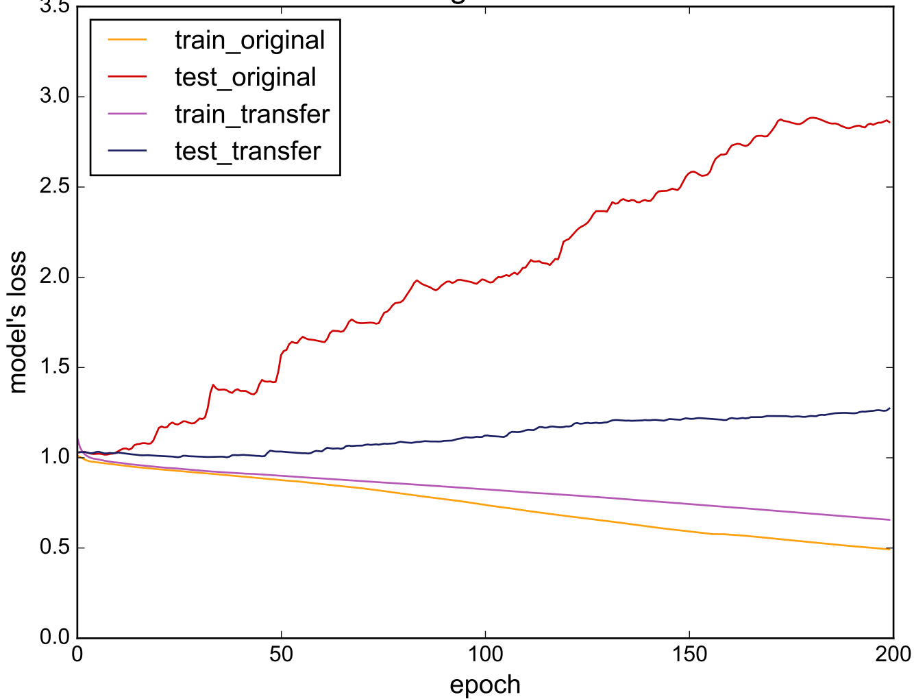
Source: OliveOil - Target: ChlorineConcentration
