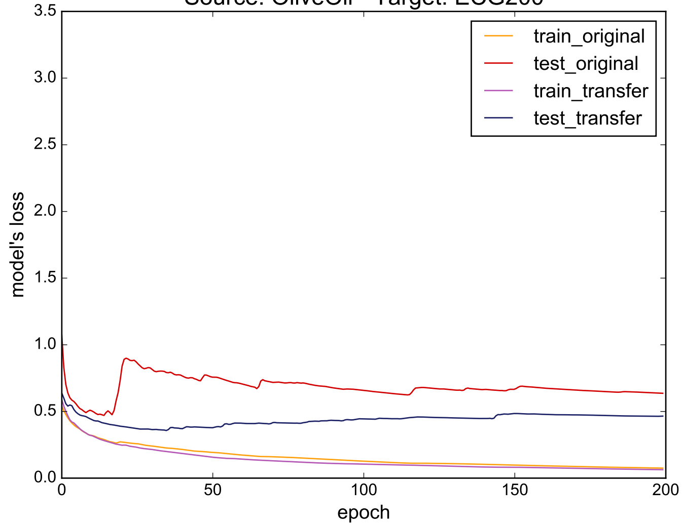
Source: OliveOil - Target: ECG200
