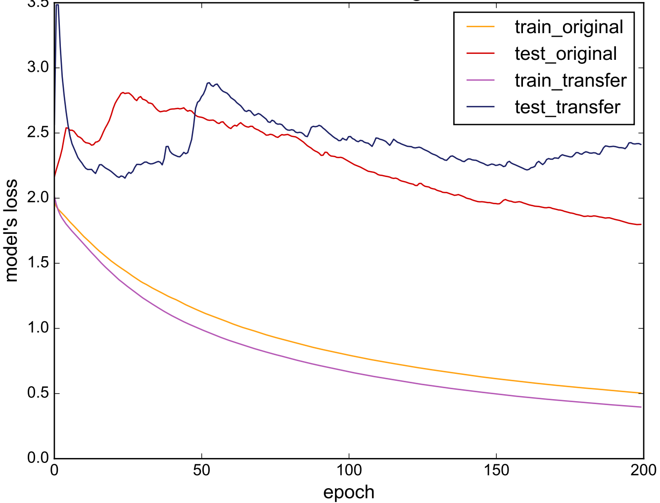
Source: OliveOil - Target: FISH
