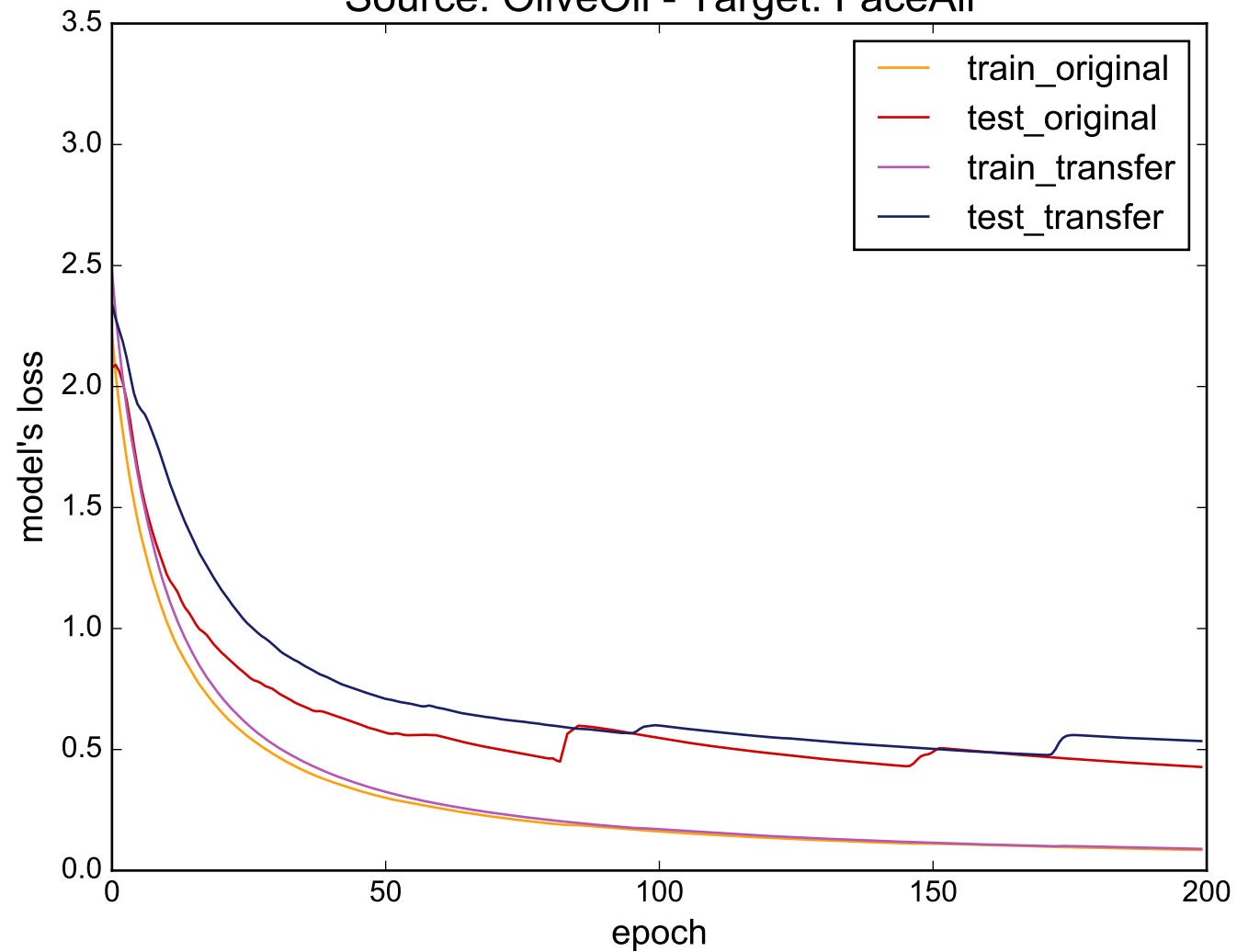
Source: OliveOil - Target: FaceAll
