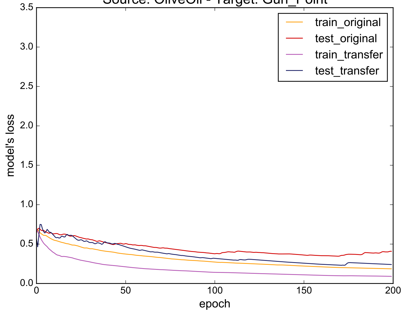
Source: OliveOil - Target: Gun_Point
