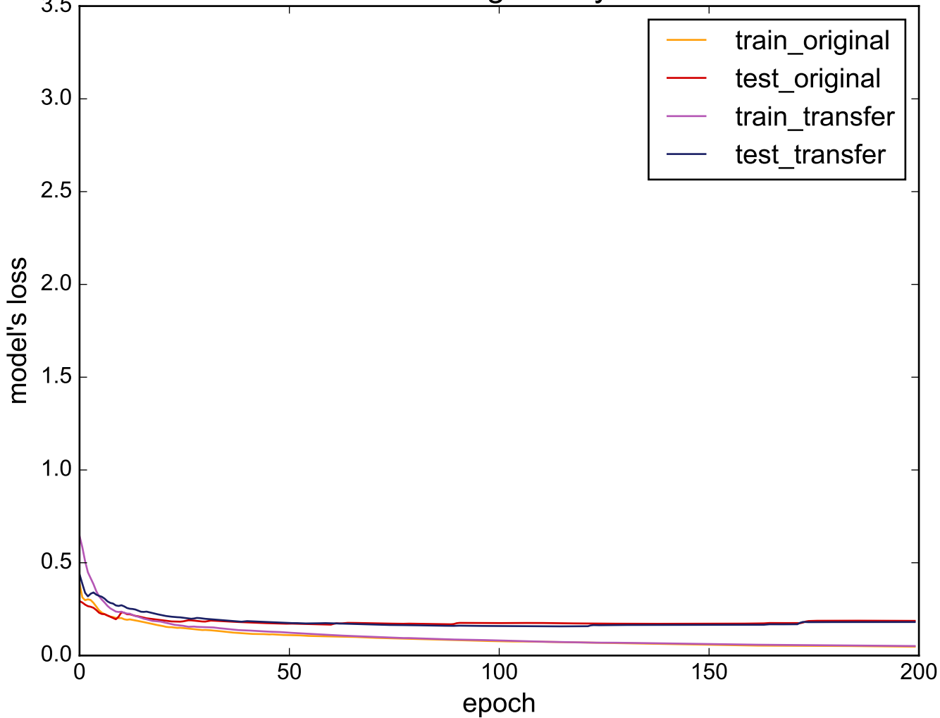
Source: OliveOil - Target: ItalyPowerDemand
