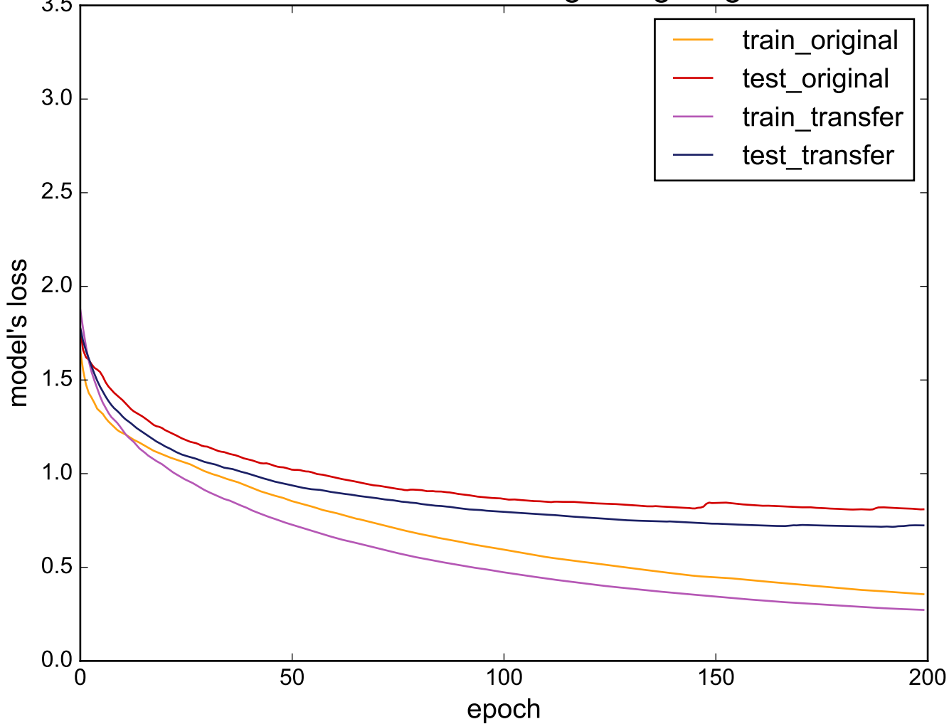
Source: OliveOil - Target: Lighting7
