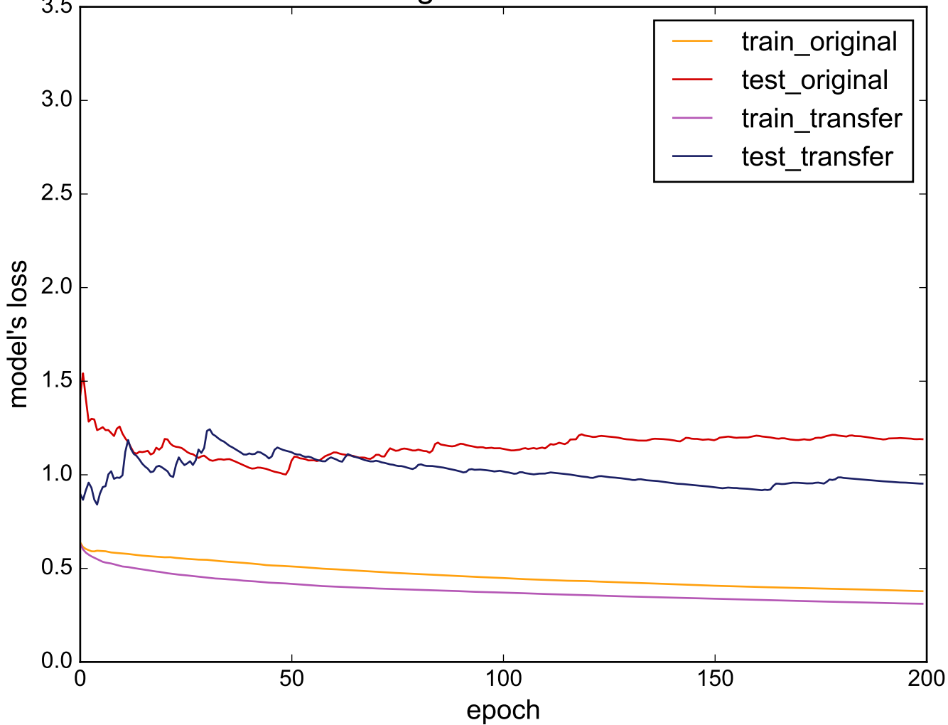
Source: OliveOil - Target: MiddlePhalanxOutlineCorrect
