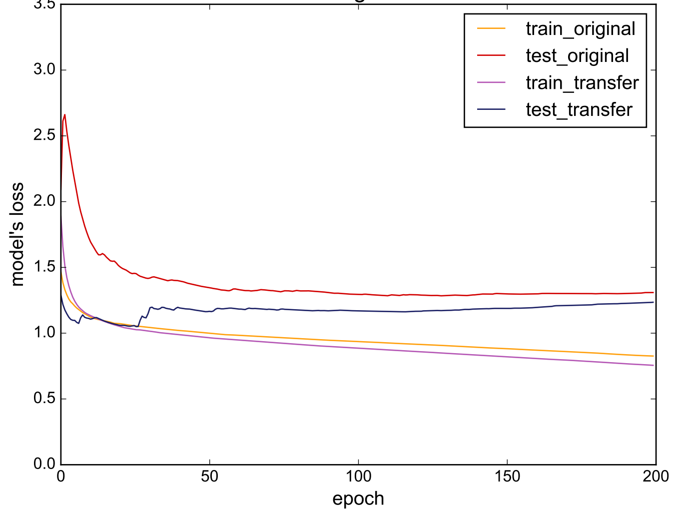
Source: OliveOil - Target: MiddlePhalanxTW
