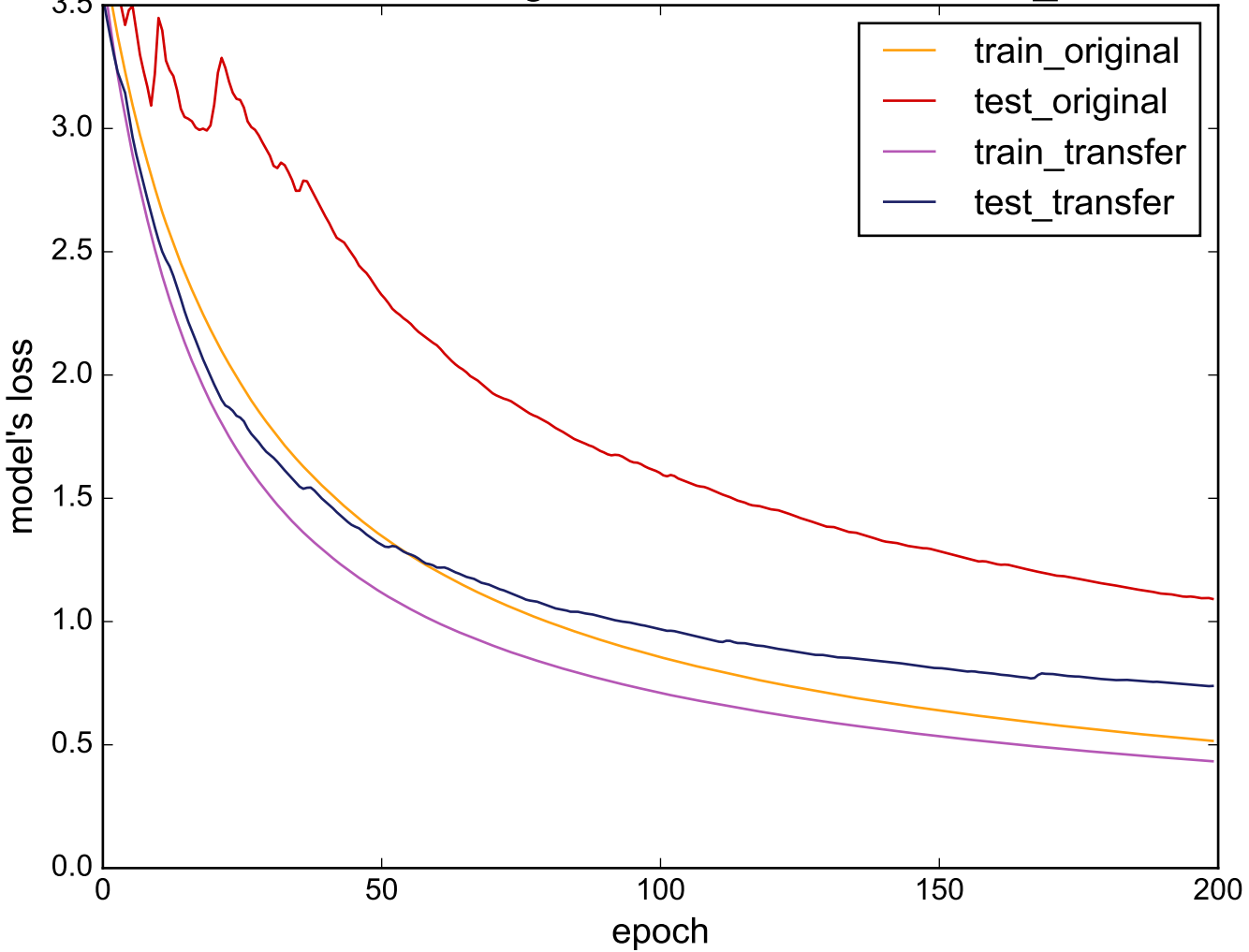
Source: OliveOil - Target: NonInvasiveFatalECG_Thorax1
