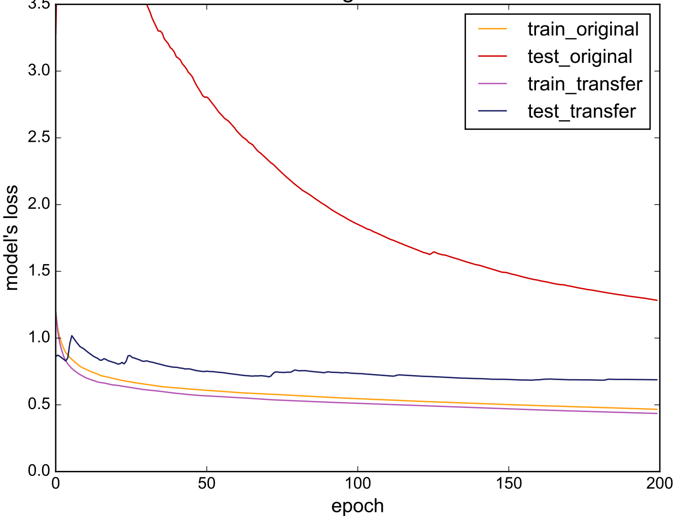
Source: OliveOil - Target: ProximalPhalanxTW
