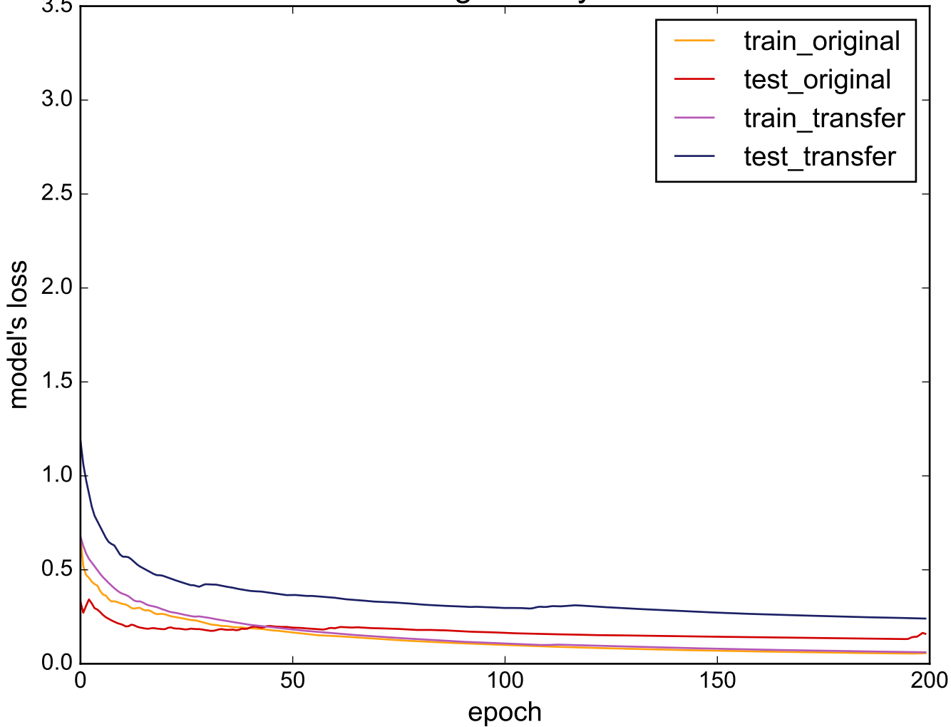
Source: OliveOil - Target: SonyAIBORobotSurface
