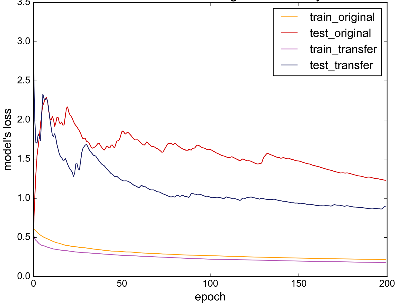
Source: OliveOil - Target: Strawberry
