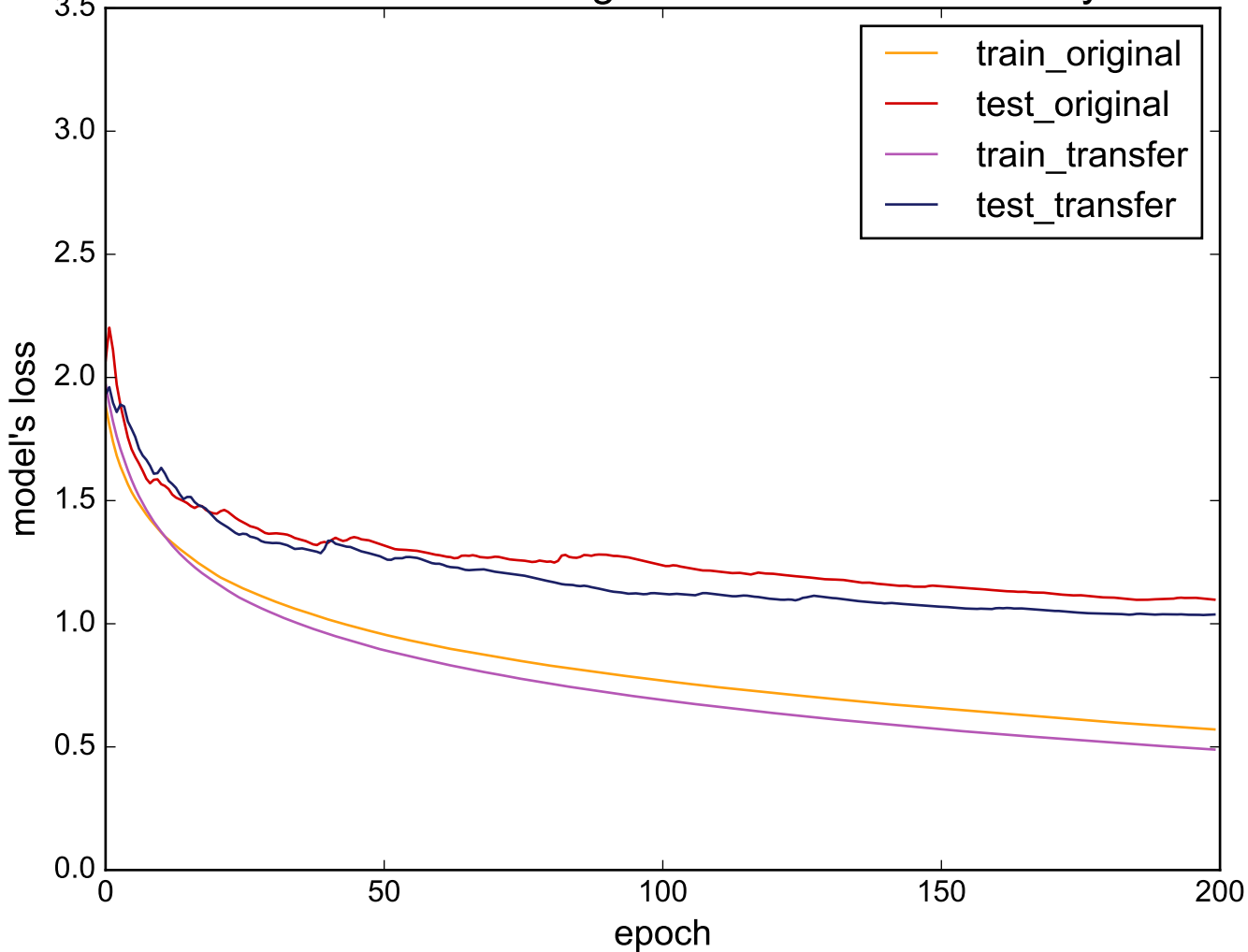
Source: OliveOil - Target: UWaveGestureLibraryAll
