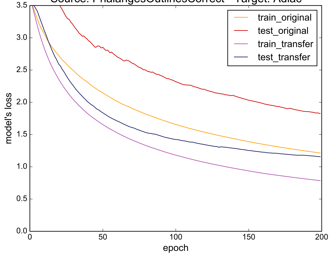
Source: PhalangesOutlinesCorrect - Target: Adiac
