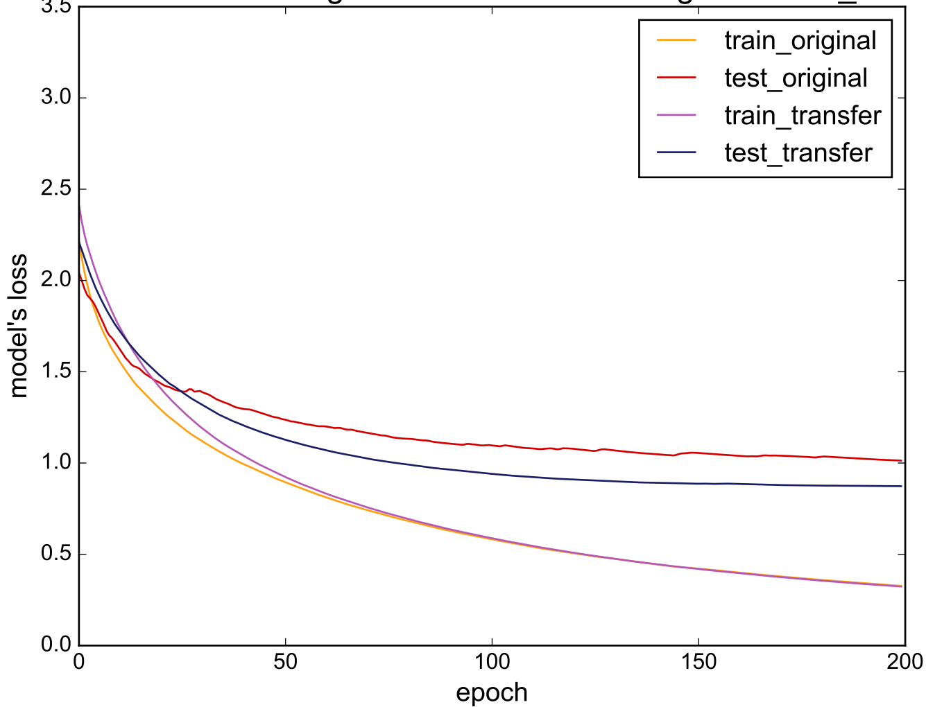
Source: PhalangesOutlinesCorrect - Target: Cricket_X
