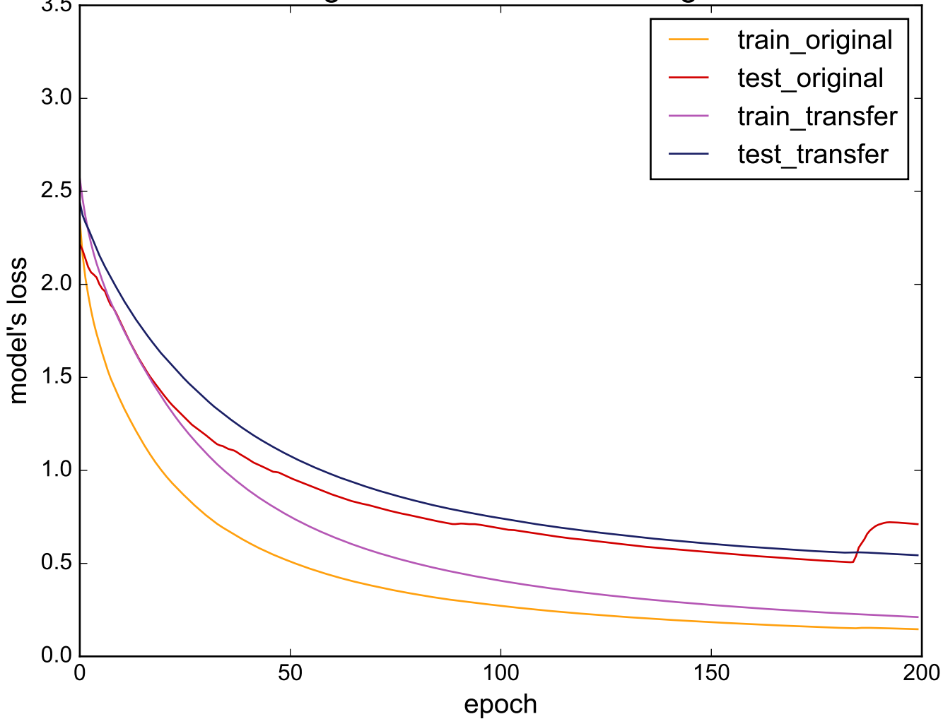
Source: PhalangesOutlinesCorrect - Target: FacesUCR
