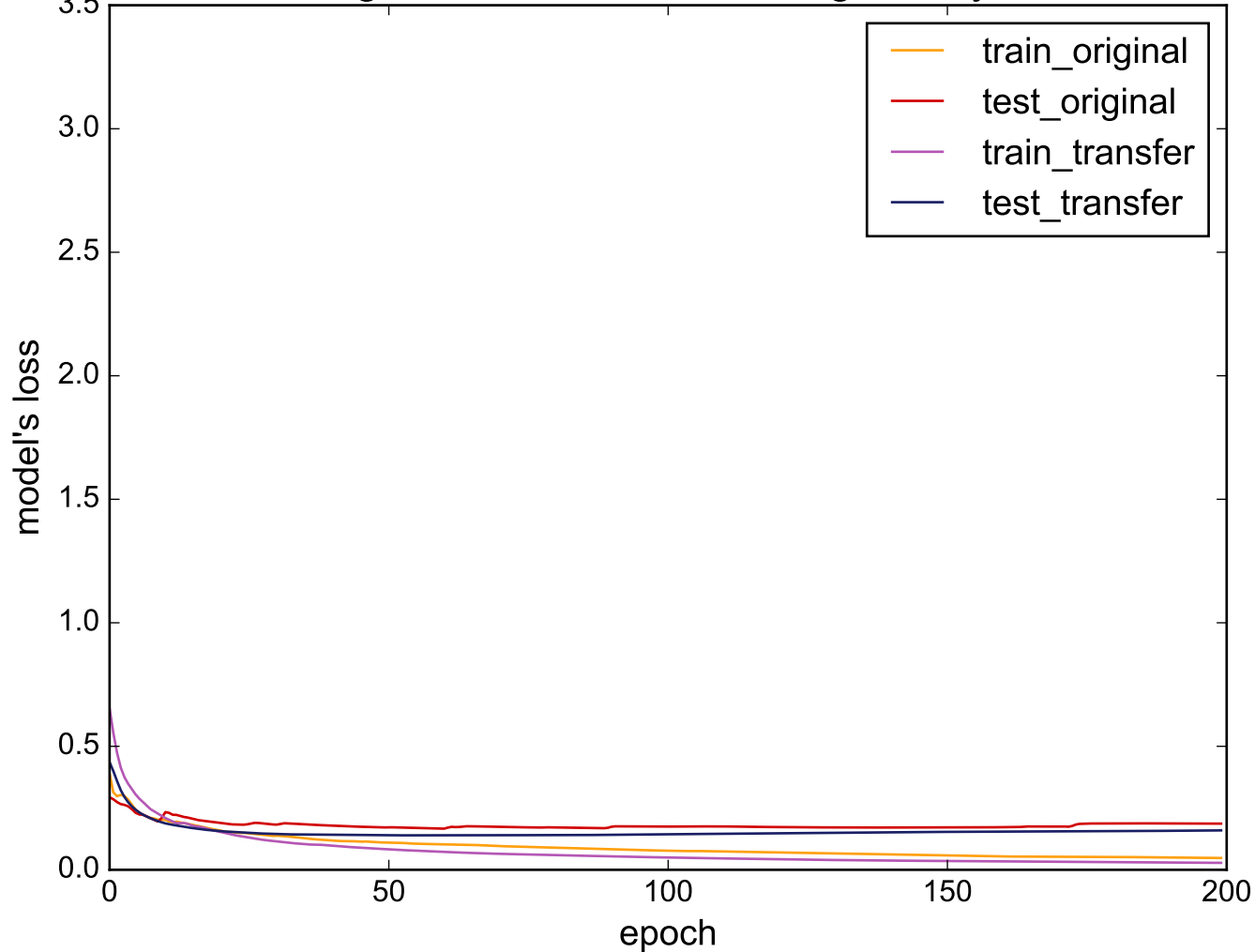
Source: PhalangesOutlinesCorrect - Target: ItalyPowerDemand
