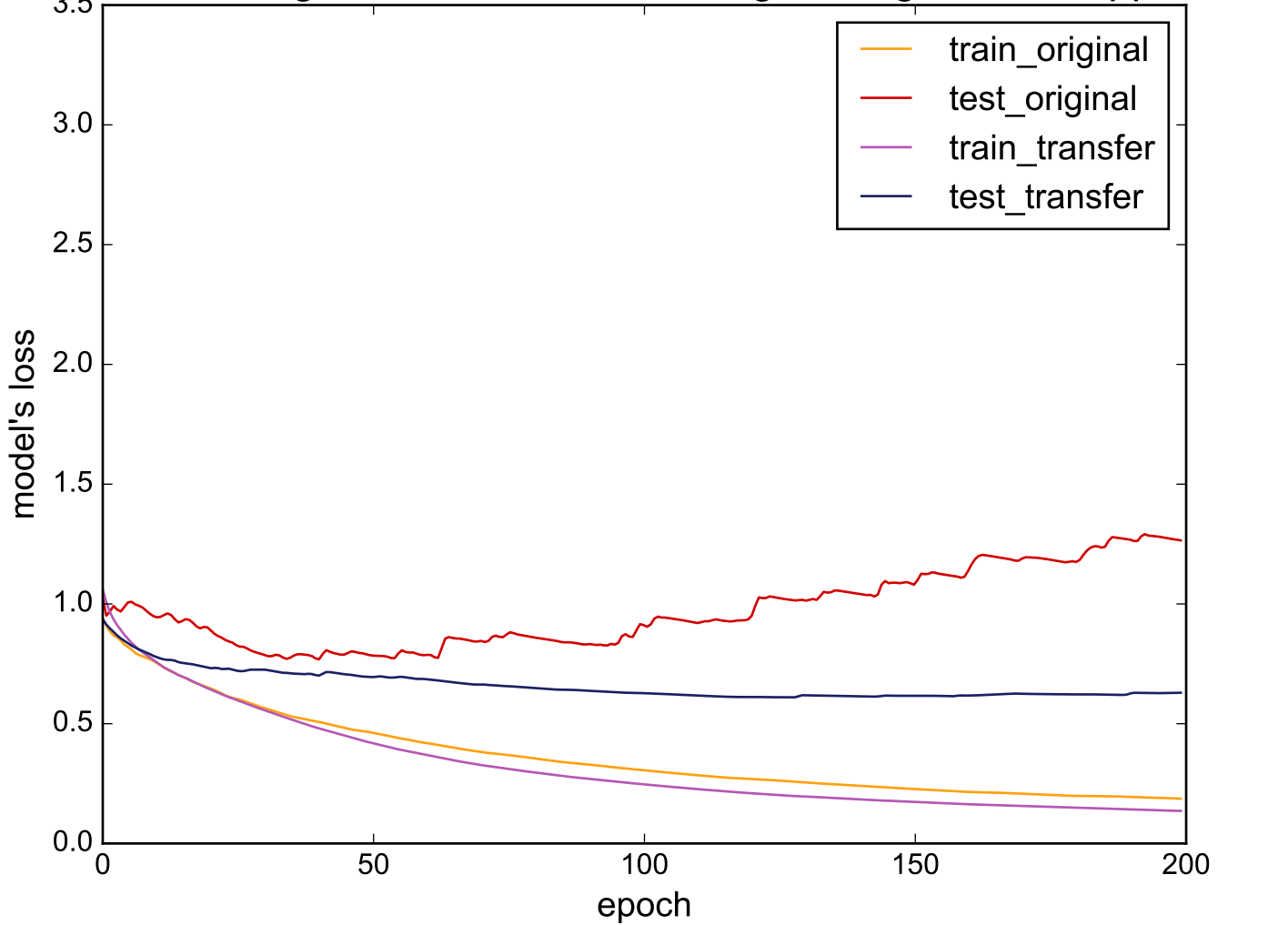
Source: PhalangesOutlinesCorrect - Target: LargeKitchenAppliances
