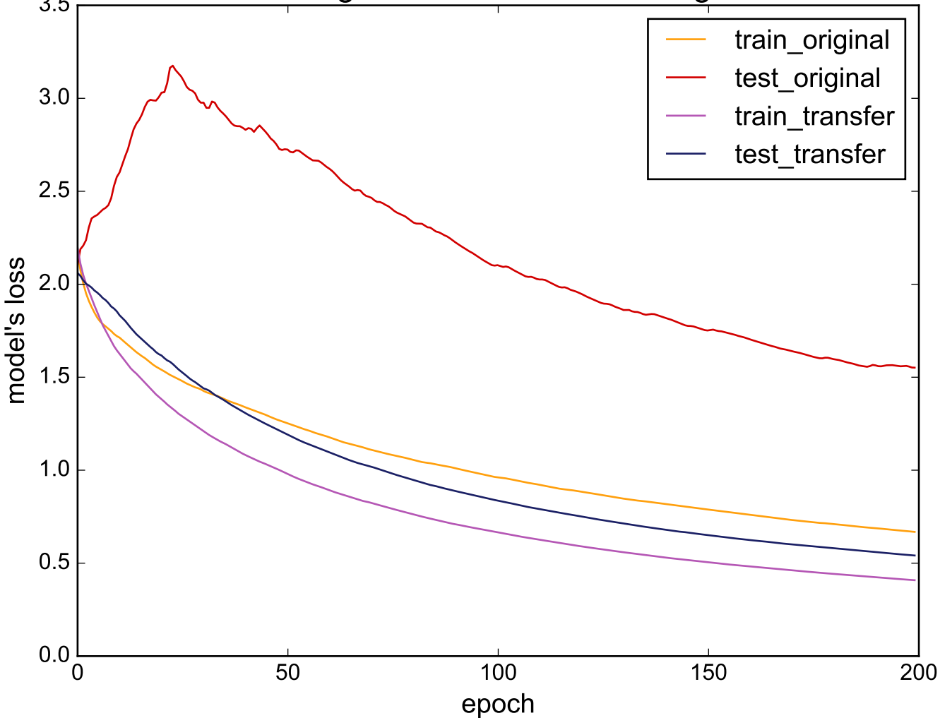
Source: PhalangesOutlinesCorrect - Target: MALLAT
