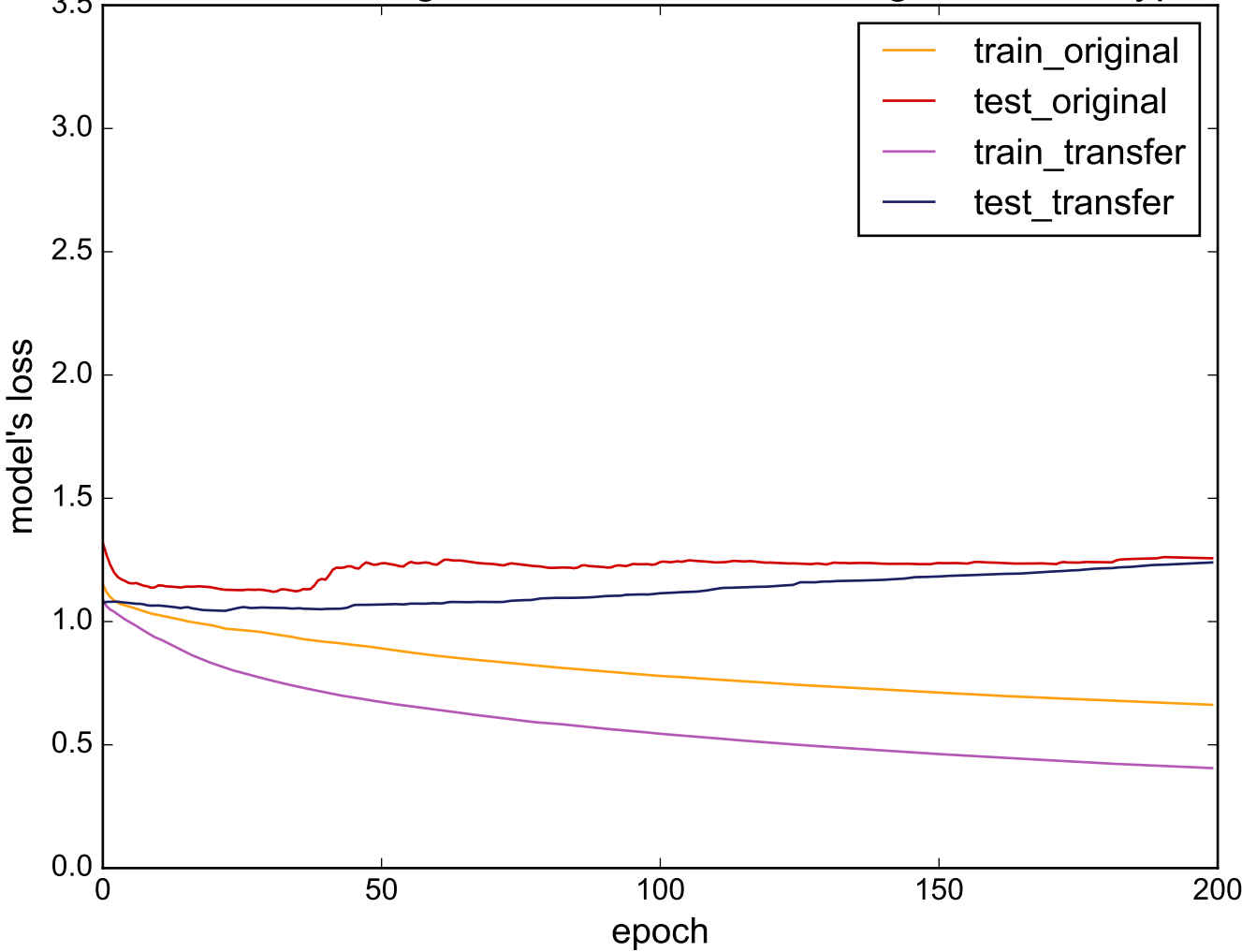
Source: PhalangesOutlinesCorrect - Target: ScreenType
