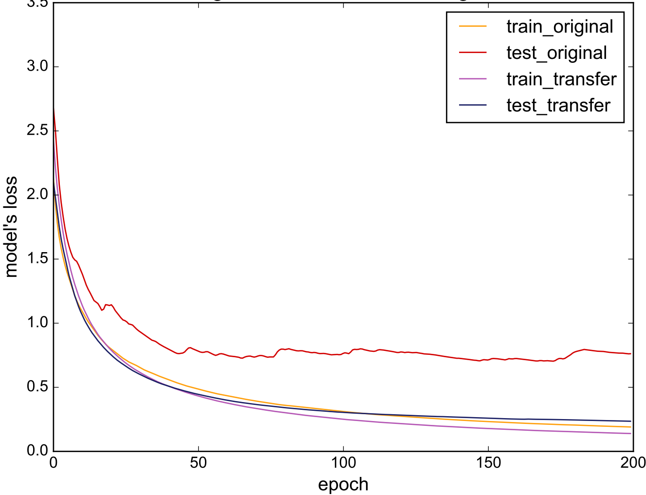
Source: PhalangesOutlinesCorrect - Target: SwedishLeaf
