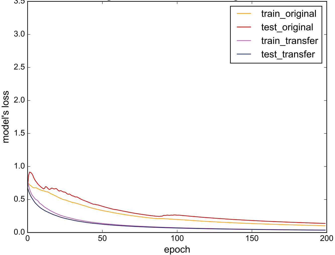
Source: PhalangesOutlinesCorrect - Target: TwoLeadECG
