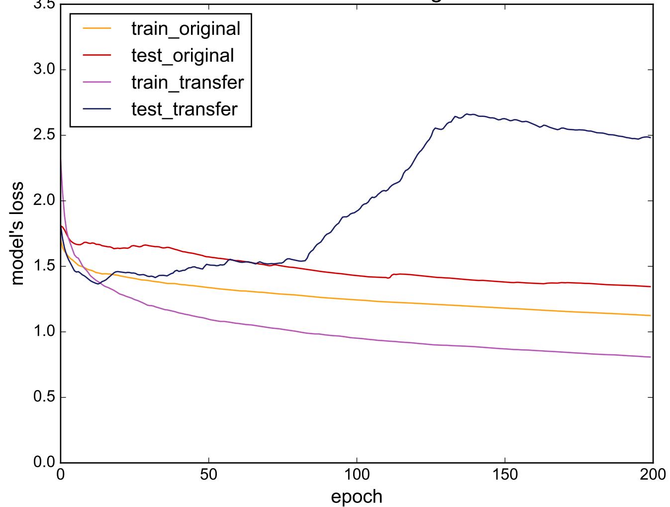
Source: Phoneme - Target: Beef
