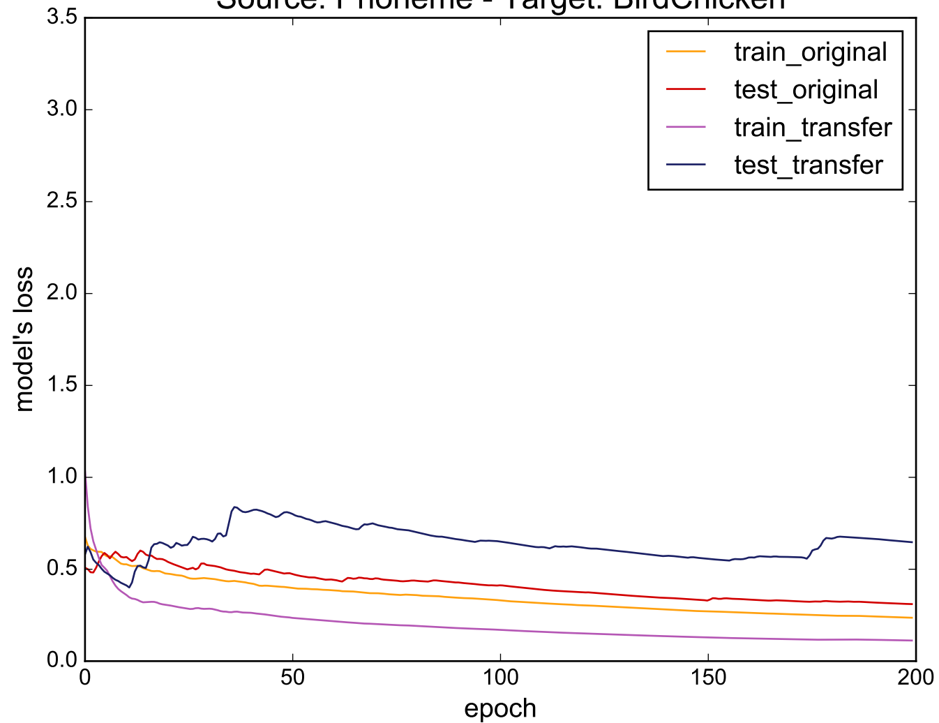
Source: Phoneme - Target: BirdChicken
