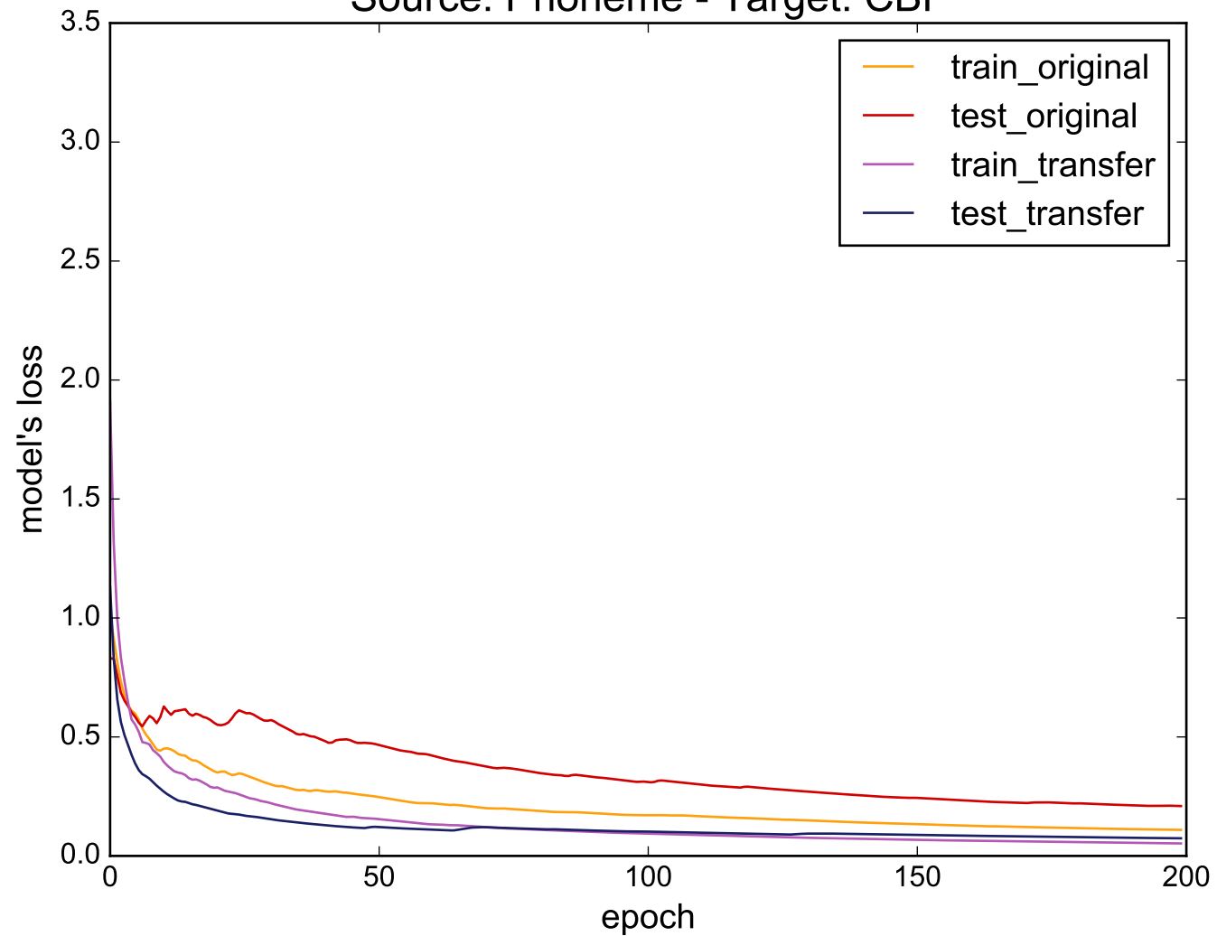
Source: Phoneme - Target: CBF
