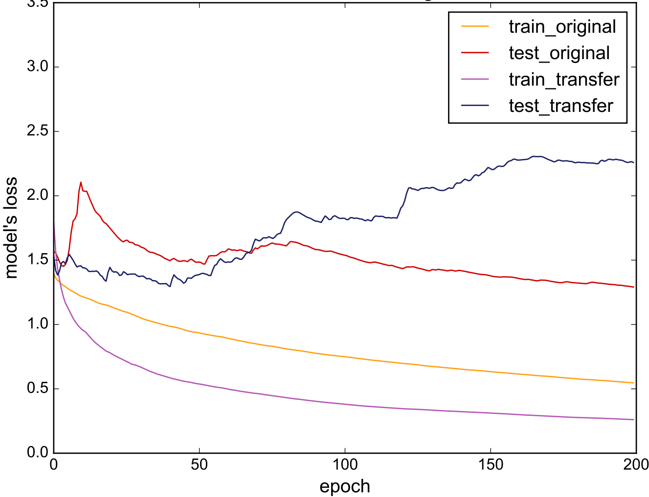
Source: Phoneme - Target: Car
