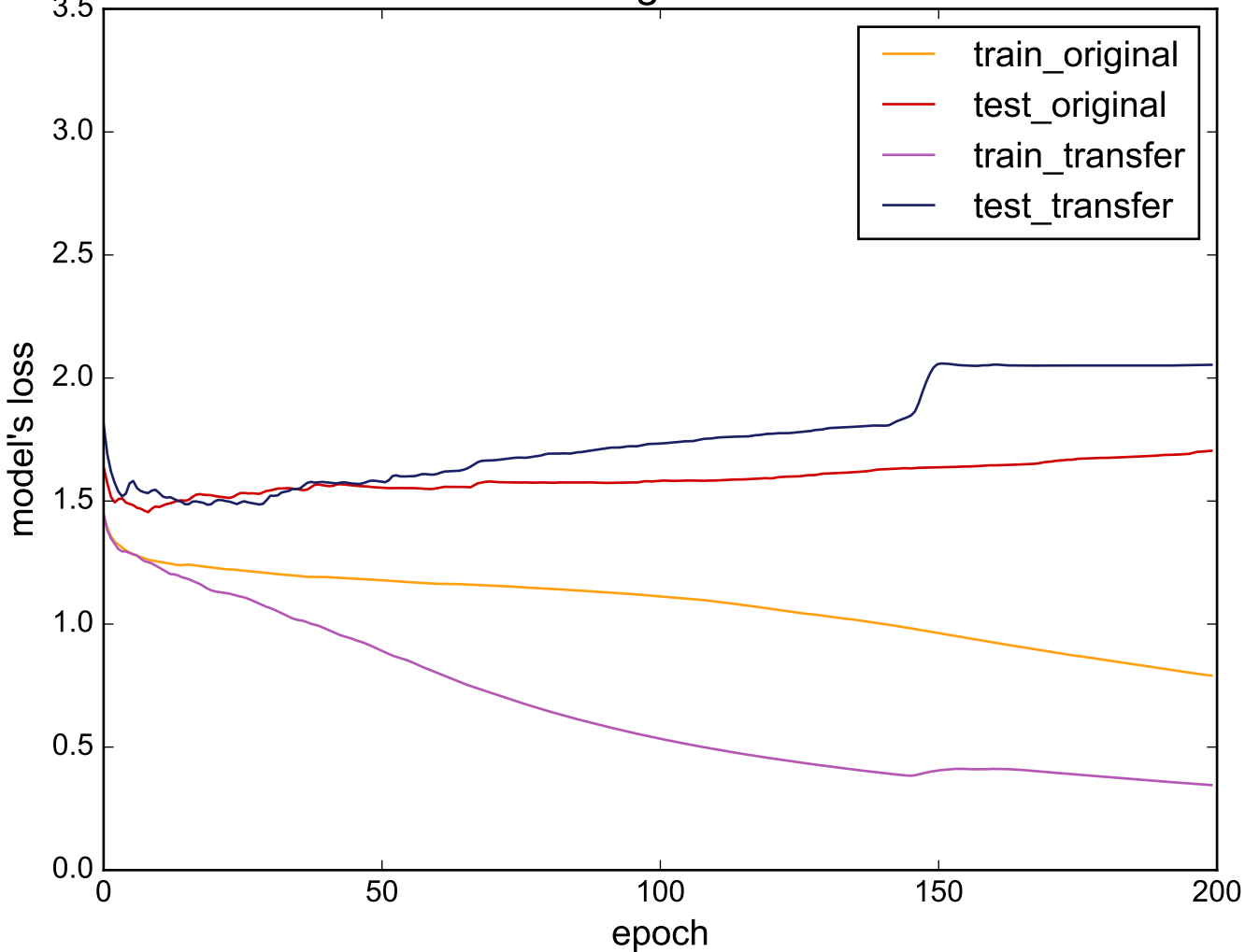
Source: Phoneme - Target: DiatomSizeReduction
