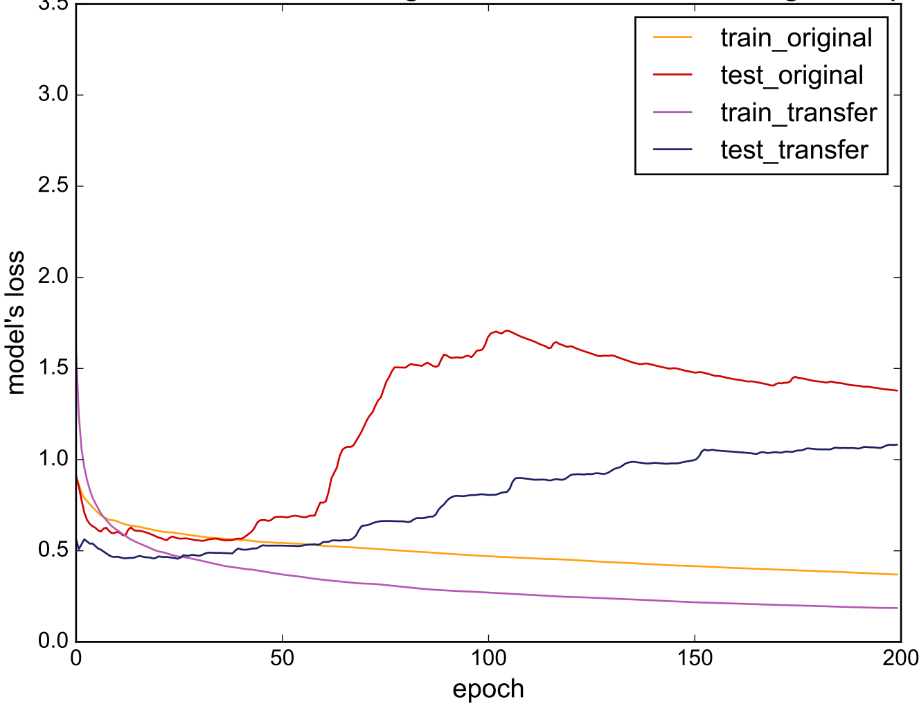
Source: Phoneme - Target: DistalPhalanxOutlineAgeGroup
